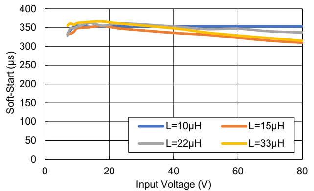
Figure 38. Soft-Start (No Load): RAA211805
