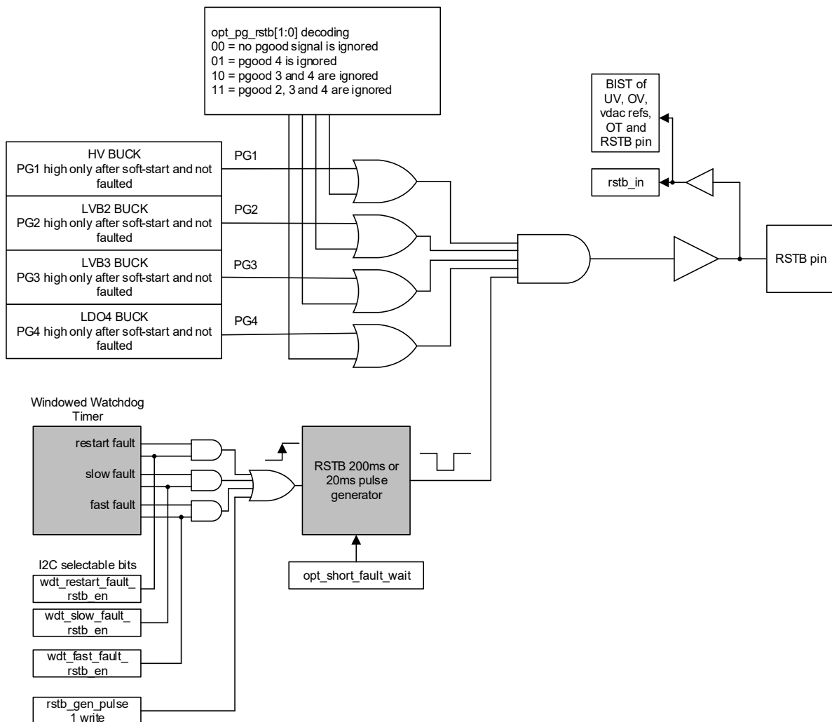
Figure 27. RSTB Block Diagram
