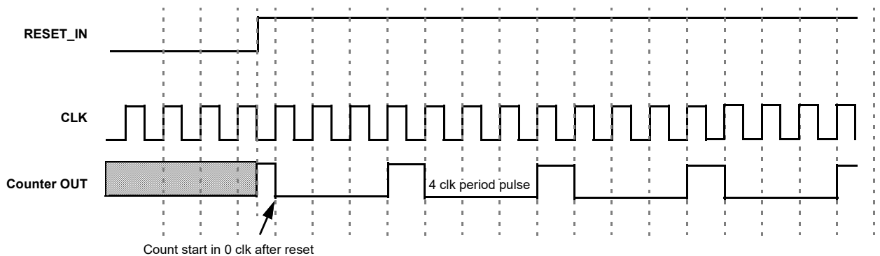
Figure 32. Counter Mode Timing Diagram
