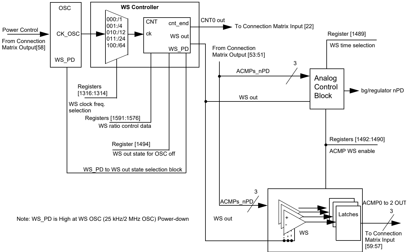
Figure 44. Wake/Sleep Controller
