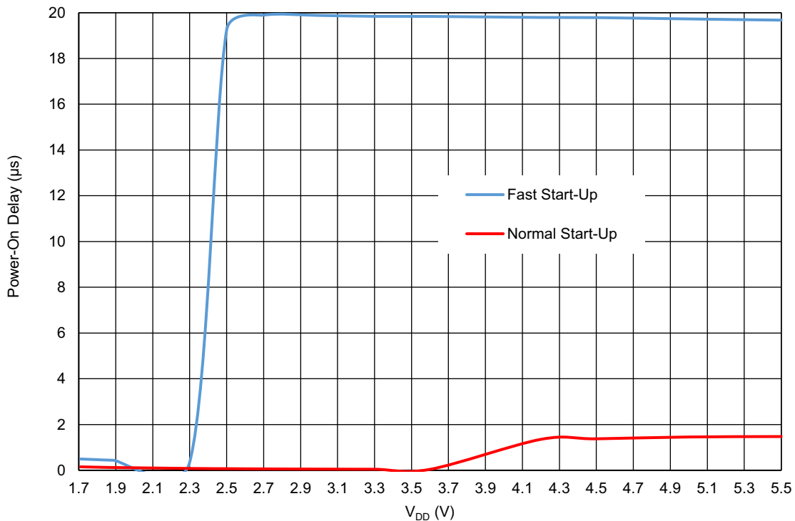
Figure 65. Oscillator Maximum Power-On Delay vs. V DD at T A = +25 °C, OSC0 = 25 kHz
