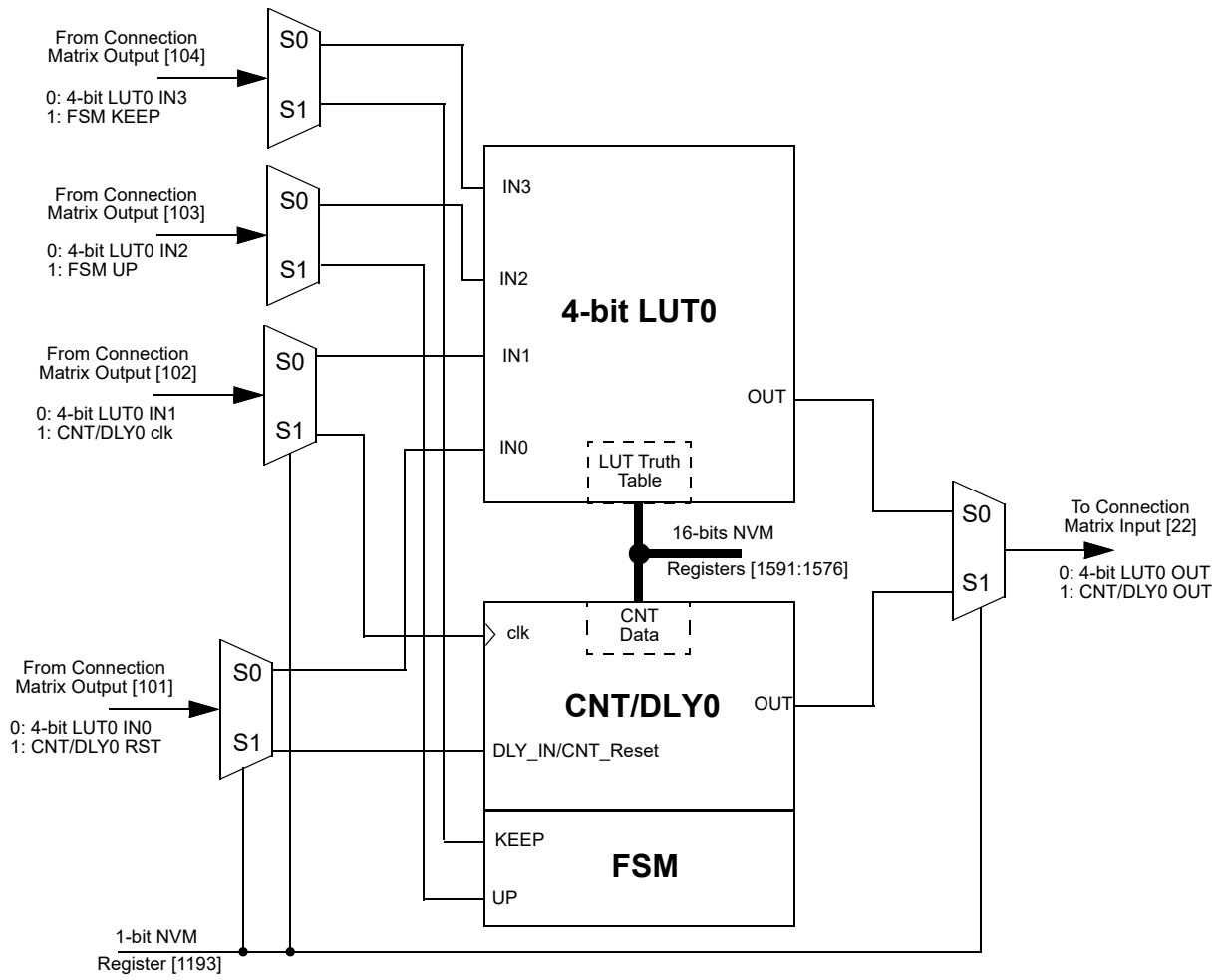
Figure 29. 4-bit LUT0 or CNT/DLY0
