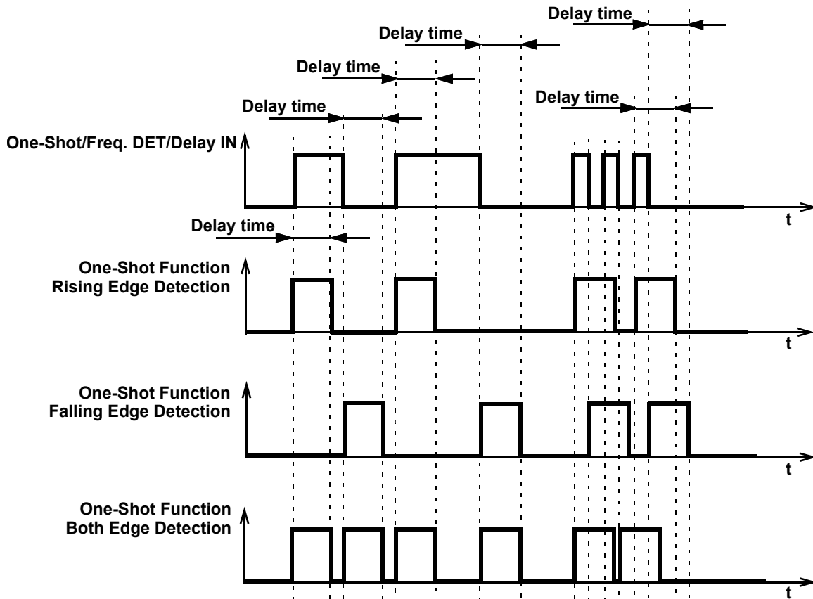
Figure 33. One-Shot Function Timing Diagram
