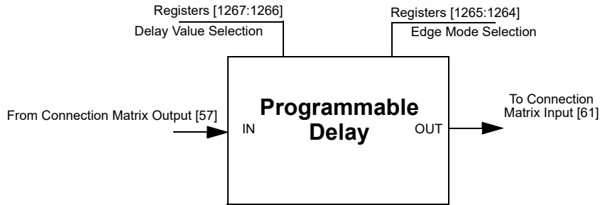
Figure 55. Programmable Delay
