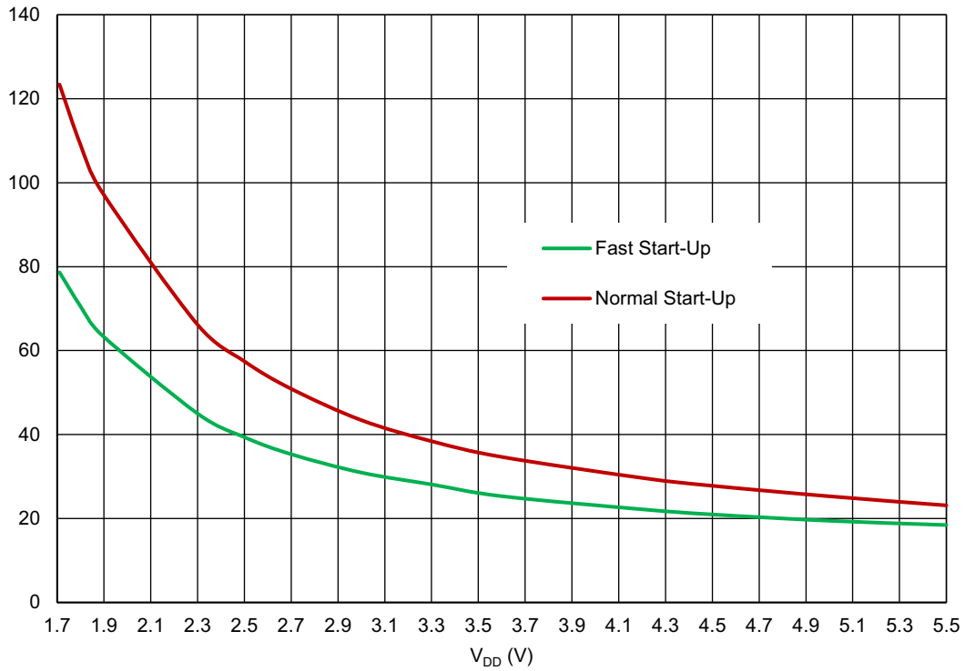
Figure 66. Oscillator Maximum Power-On Delay vs. V DD at T A = +25 °C, OSC0 = 2 MHz
