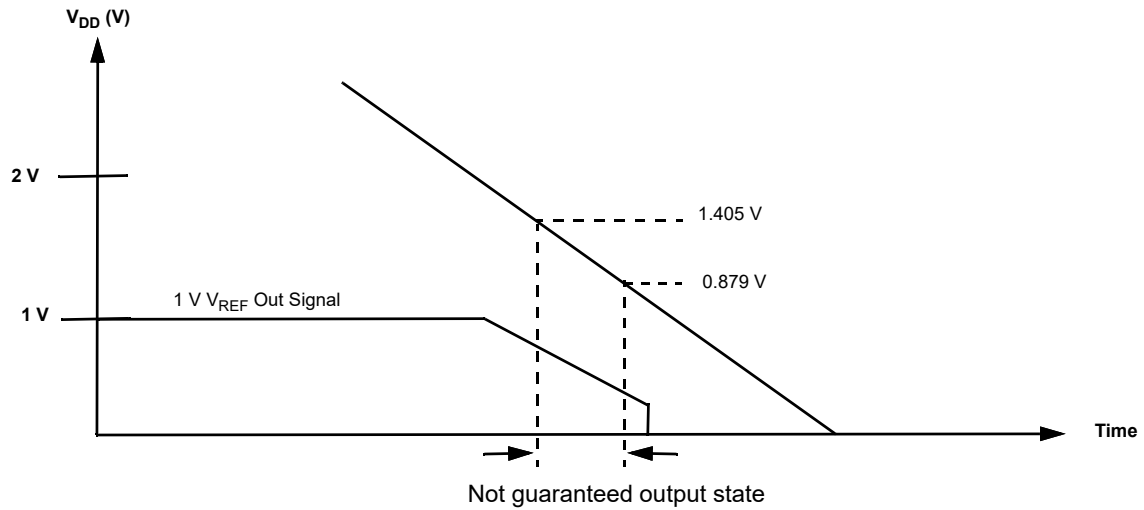
Figure 86. Power-Down
