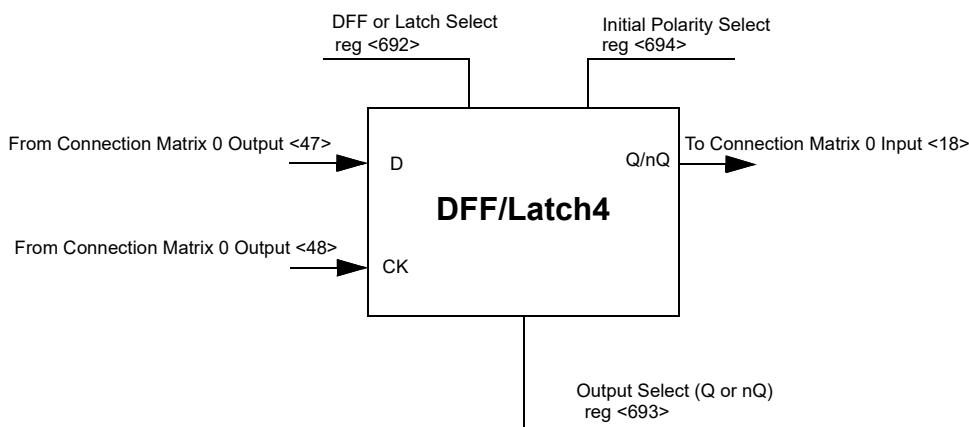
Figure 66. DFF/Latch4
