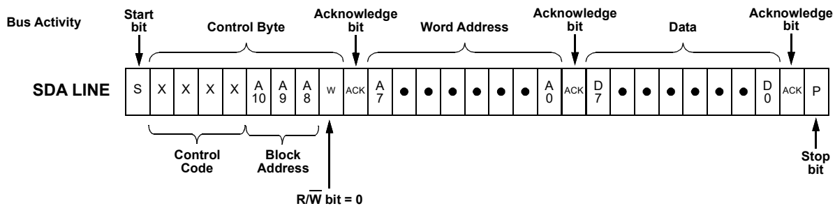
Figure 238: Byte Write Command, R/\bar{W} = 0
