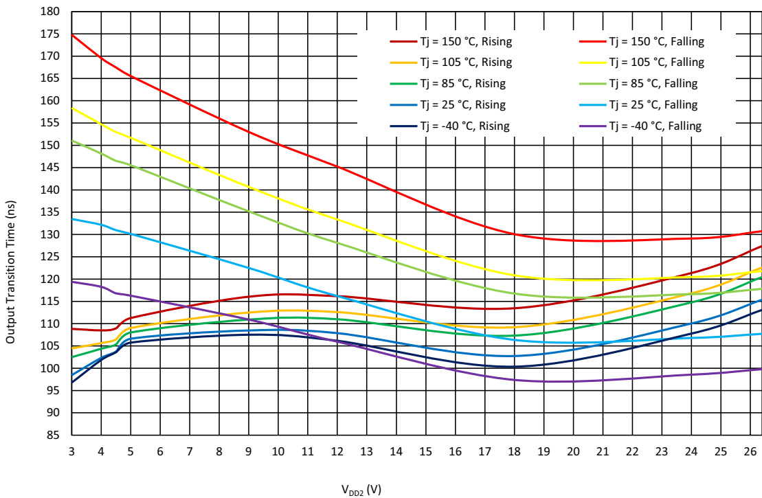
Figure 32. Half Bridge Output Transition Time vs. V DD2 at V DD = 2.3 V to 5.5 V, f = 50 kHz for Regular Mode
