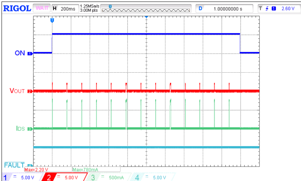
Figure 22. Typical SOA waveform during powerup on heavy load for V_{IN} = 9\text{ V} , C_{LOAD} = 10\text{ }\mu\text{F} , R_{SET} = 30.1\text{ k}\Omega , R_{LOAD} = 3.8\text{ }\Omega
