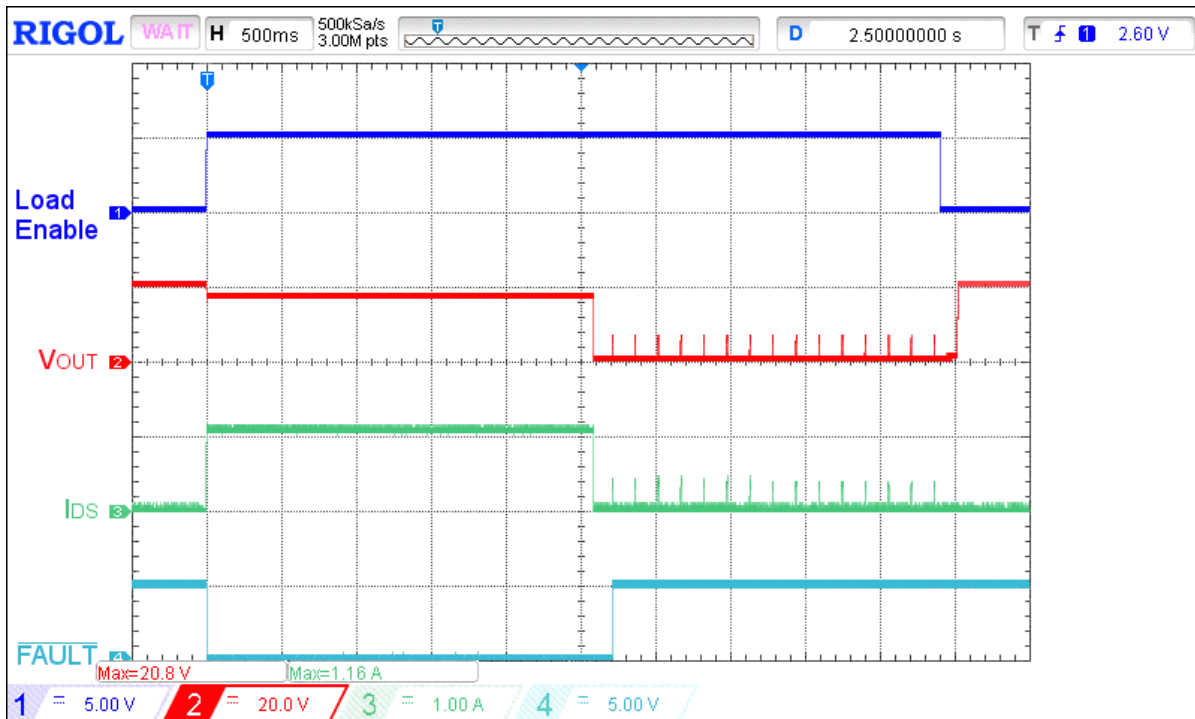
Figure 21. Thermally induced SOA shutdown for V_{IN} = 20\text{ V} , C_{LOAD} = 10\text{ }\mu\text{F} , I_{ACL} = 1\text{ A} , R_{SET} = 91\text{ k}\Omega
