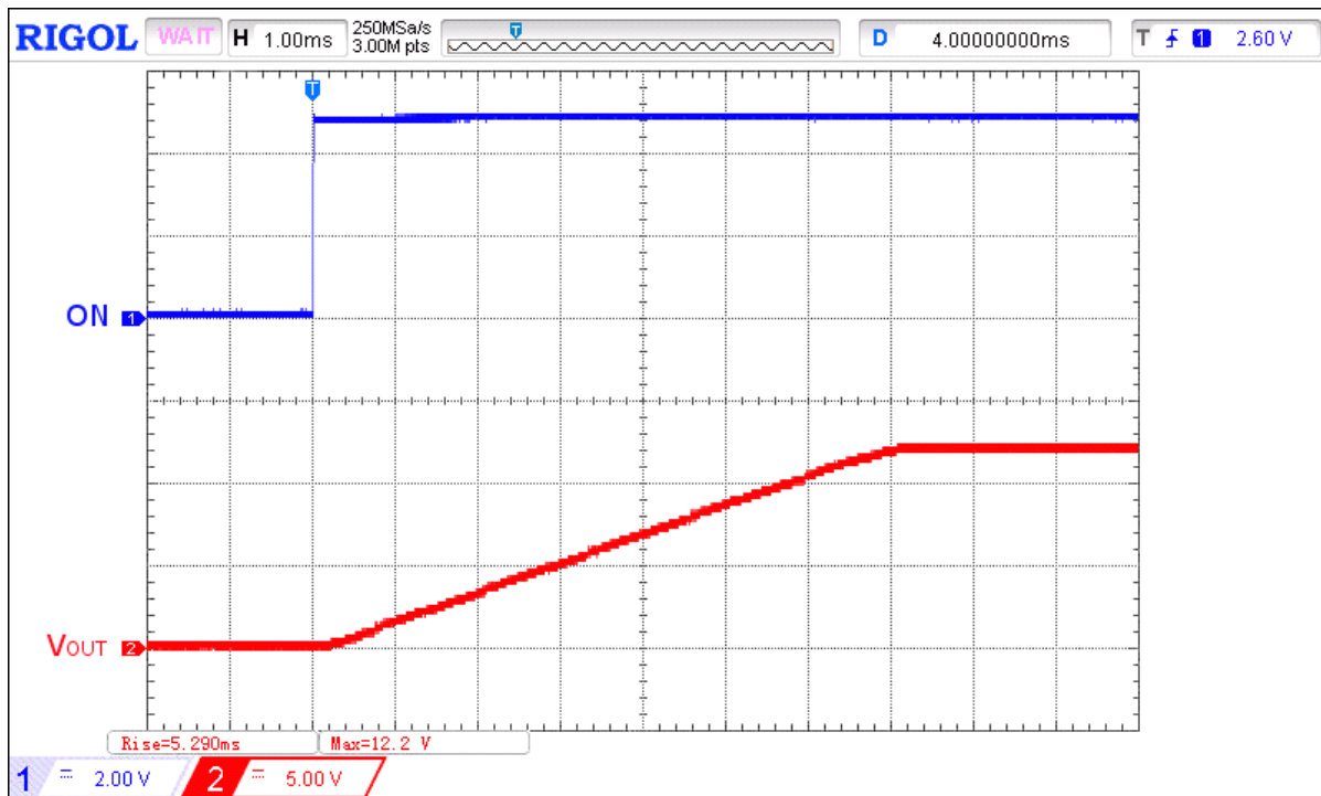
Figure 3. Typical Turn ON operation waveform for V_{IN} = 12V , C_{SLEW} = 18nF , C_{LOAD} = 10\mu F , R_{LOAD} = 100\Omega
