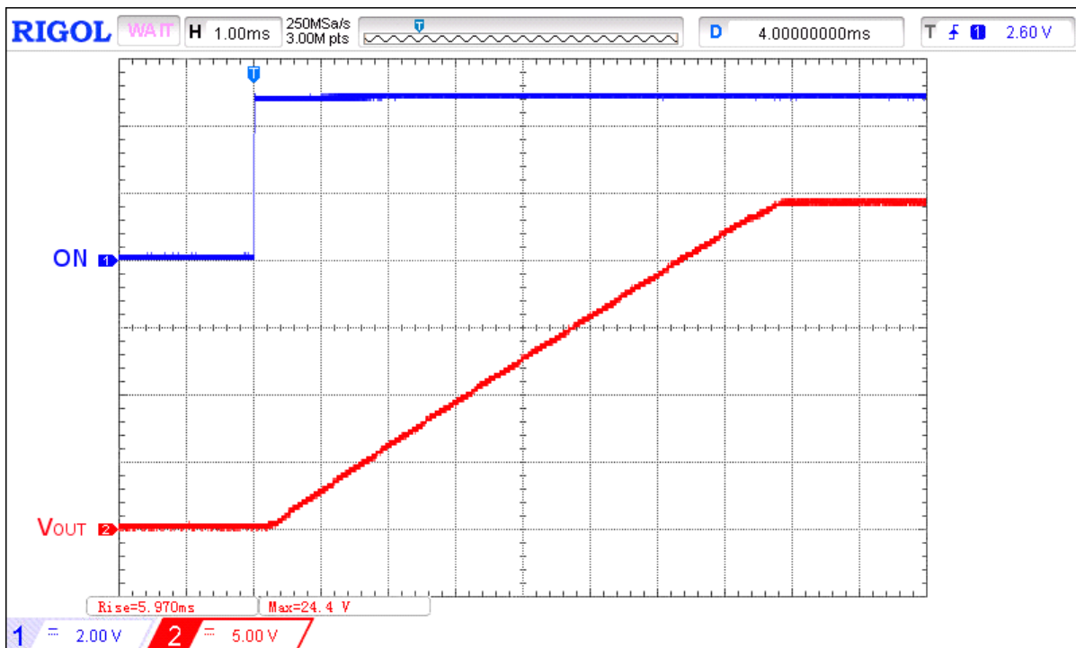
Figure 4. Typical Turn ON operation waveform for V_{IN} = 24V , C_{SLEW} = 10nF , C_{LOAD} = 10\mu F , R_{LOAD} = 100\Omega
