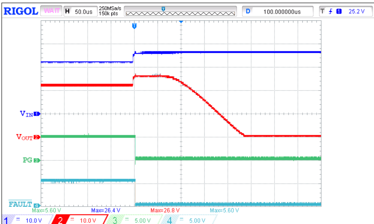
Figure 32. OVLO Operation Waveform for V_{IN} = 22 \text{ V} \rightarrow 26 \text{ V}
