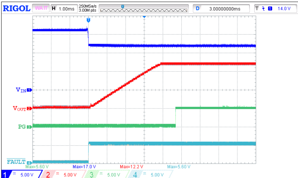
Figure 31. OVLO Operation Waveform for V_{IN} = 16 \text{ V} \rightarrow 12 \text{ V}
