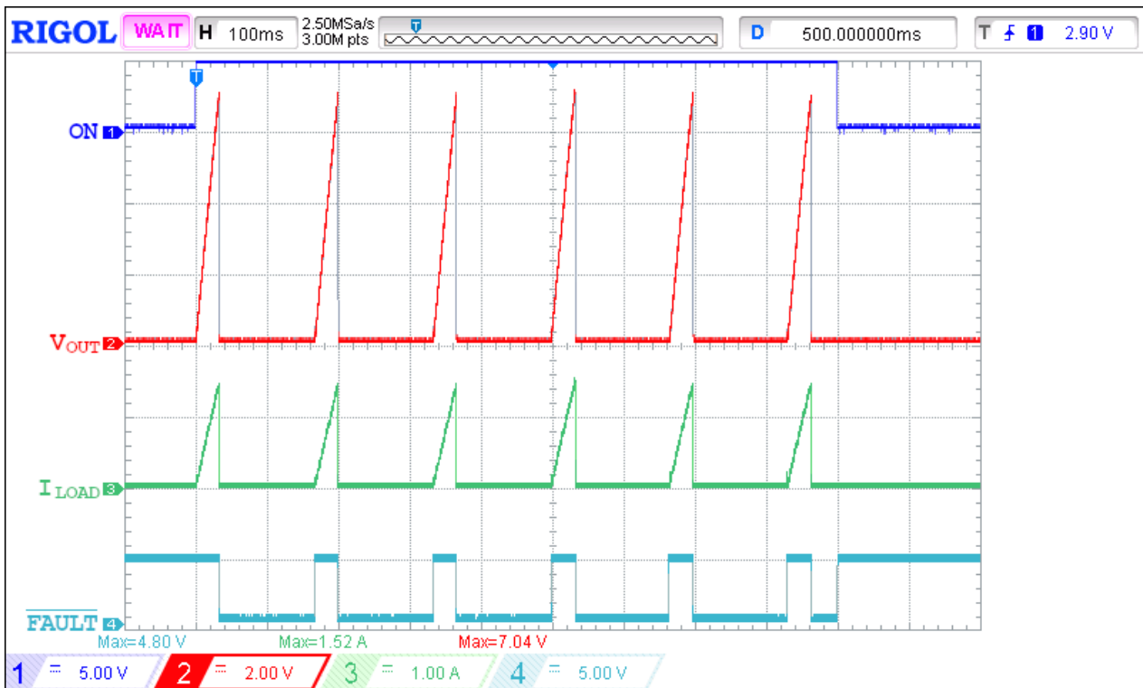
Figure 49. 12.5 W SOA Protection Operation Waveform with 18 ms Blanking Time for V_{IN} = 22 \text{ V}
