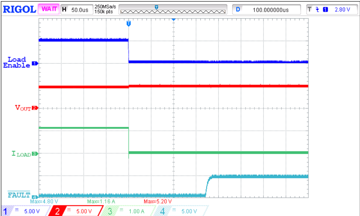
Figure 40. FAULT De-Assertion Operation Waveform for V IN = 4.5 V, Switch Out 3.9 Ω Load
