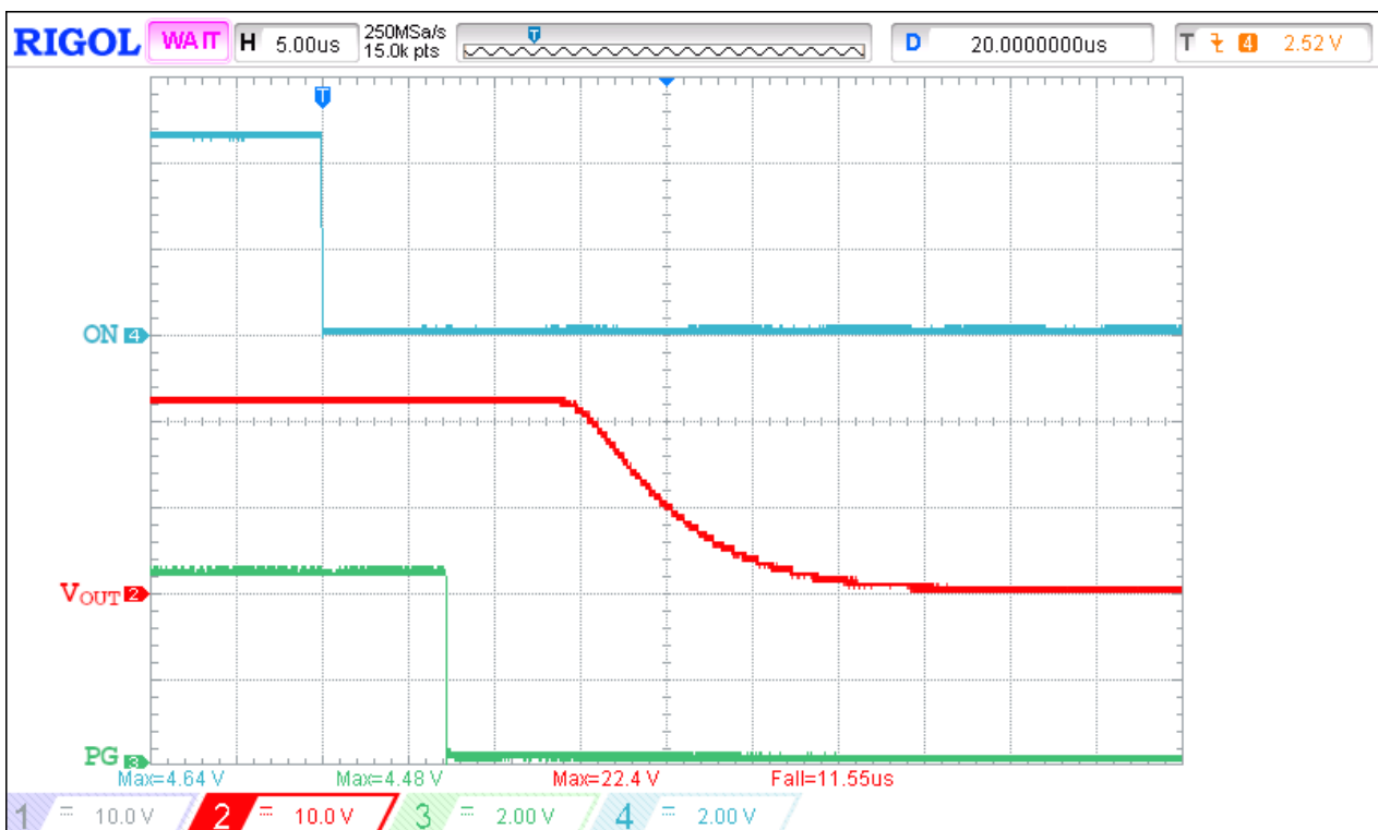
Figure 28. Turn OFF Operation Waveform for V_{IN} = 22\text{ V}
