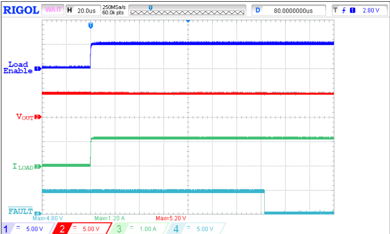
Figure 39. FAULT Assertion Operation Waveform for V IN = 4.5 V, Switch In 3.9 Ω Load
