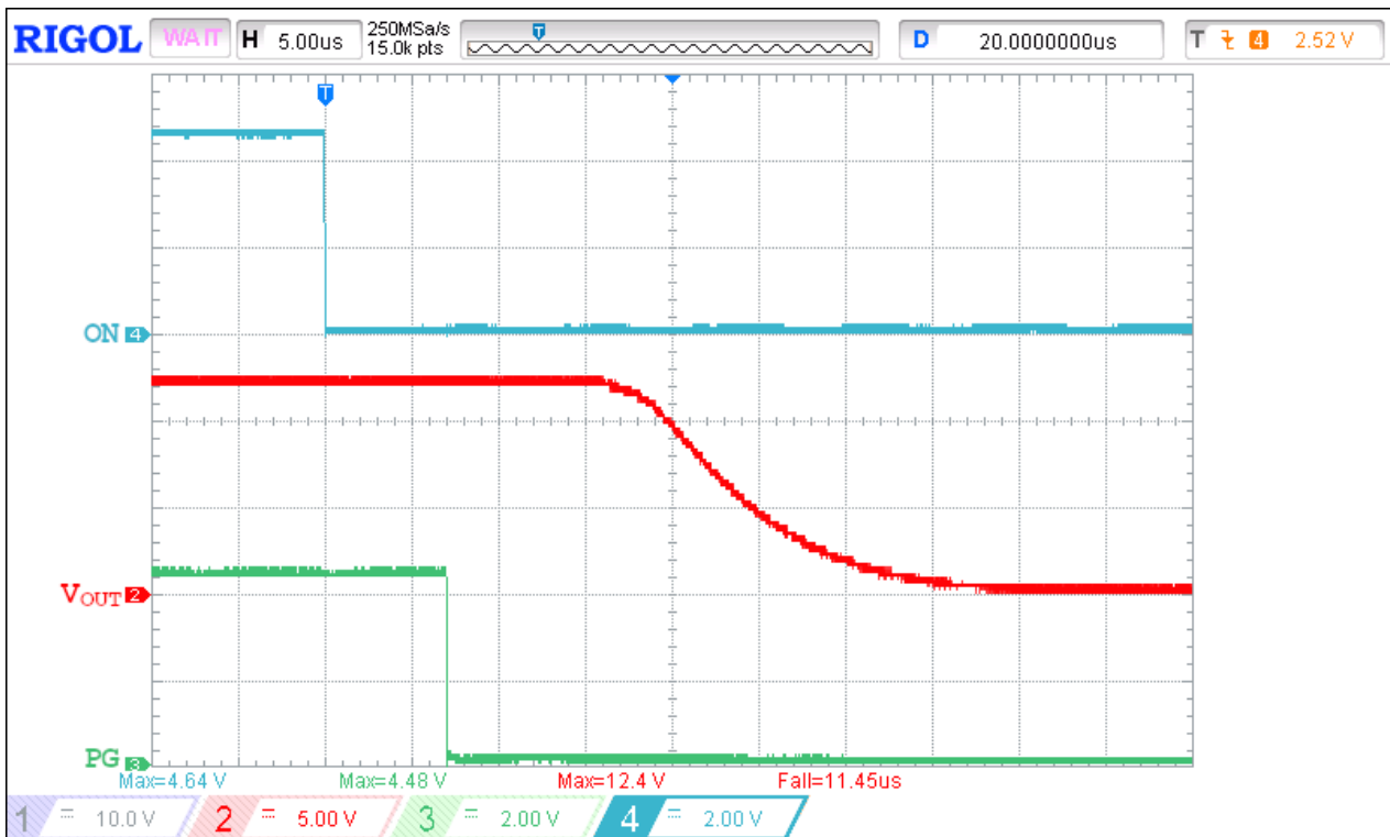
Figure 27. Turn OFF Operation Waveform for V_{IN} = 12\text{ V}
