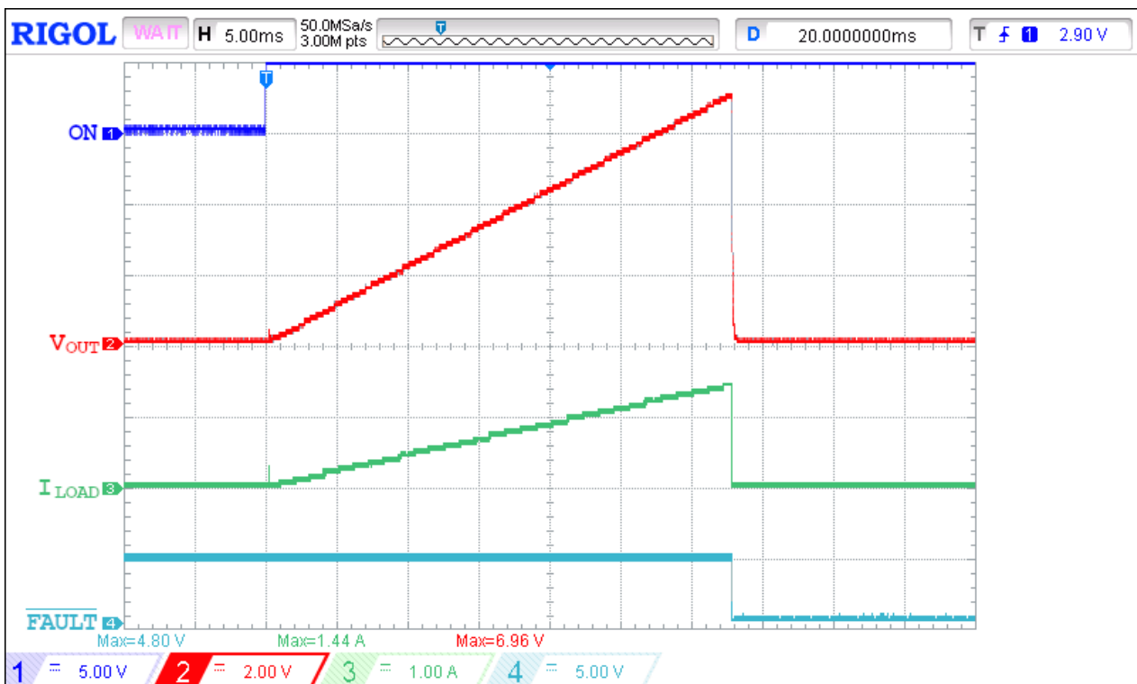
Figure 50. 12.5 W SOA Protection Operation Waveform with 18 ms Blanking Time for V_{IN} = 22 \text{ V} (Extended View)
