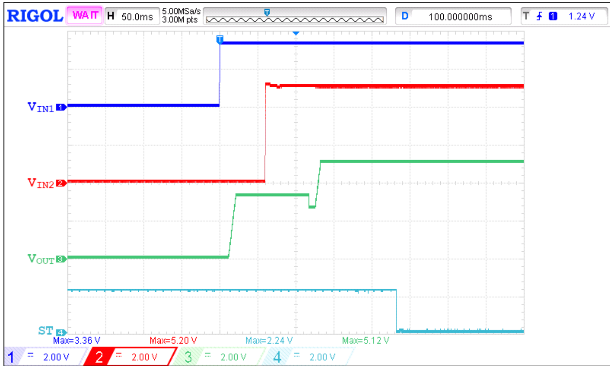
Figure 11. Higher voltage level priority operation waveform for V_{IN1} = 3.3 \text{ V} , V_{IN2} = 5 \text{ V} , SEL = 0 \text{ V} , PR = 0 \text{ V} , C_{SS} = 220 \text{ nF} , R_{LOAD} = 100 \Omega , C_{LOAD} = 2 \mu\text{F}
