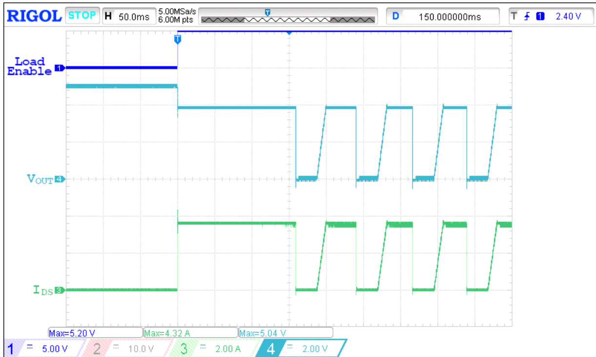
Figure 17. Active Current Limit operation waveform for V_{IN[1,2]} = 5\text{ V} , C_{SS} = 220\text{ nF} , R_{LIM} = 31.6\text{ k}\Omega , R_{LOAD} = 1.1\ \Omega , C_{LOAD} = 2\ \mu\text{F}
