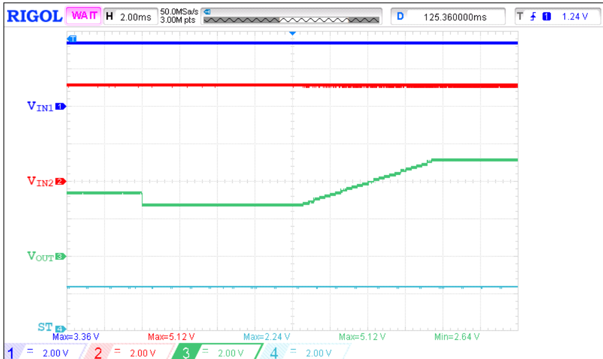
Figure 12. Higher voltage level priority operation waveform for V_{IN1} = 3.3 \text{ V} , V_{IN2} = 5 \text{ V} , SEL = 0 \text{ V} , PR = 0 \text{ V} , C_{SS} = 220 \text{ nF} , R_{LOAD} = 100 \Omega , C_{LOAD} = 2 \mu\text{F} (Extended View)
