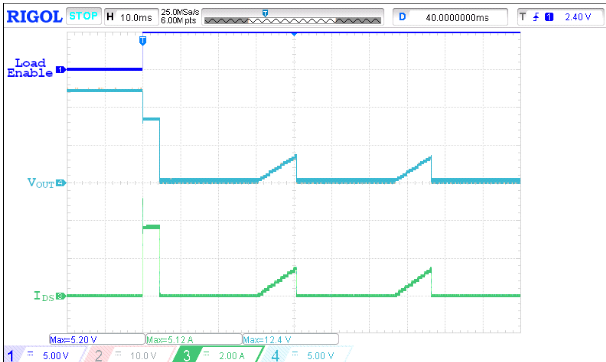
Figure 18. Active Current Limit operation waveform for V_{IN[1,2]} = 12\text{ V} , C_{SS} = 220\text{ nF} , R_{LIM} = 31.6\text{ k}\Omega , R_{LOAD} = 2.2\ \Omega , C_{LOAD} = 2\ \mu\text{F}
