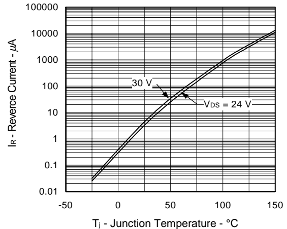
SOURCE TO DRAIN DIODE REVERSE CURRENT
