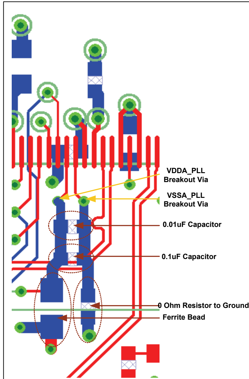
Figure 12: VDDA_PLL Filter Layout Example
