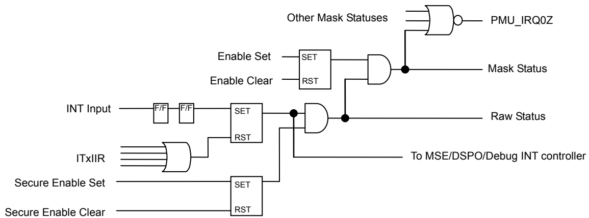
Figure F-2. Interrupt Signal Control (for Edge Detection Interrupts)
