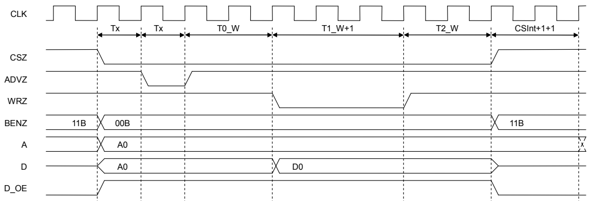
Figure E-5. Single Write Timing (AD-Mux) ( T_0 > 0 ) (Clock Ratio = 1:1)
