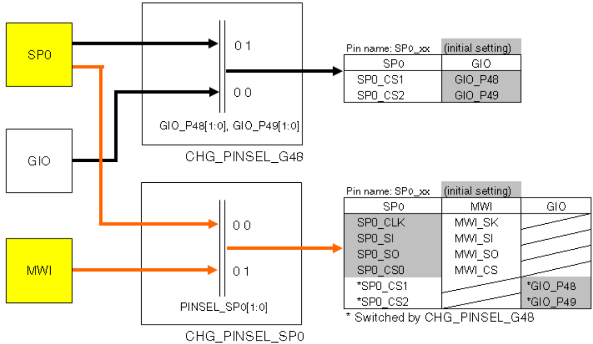
Figure 8-5. Selector Configuration of SPI0/MWI Interface Alternate-Function Pins
