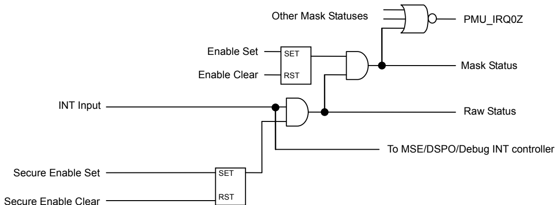
Figure F-1. Interrupt Signal Control (for Level Detection Interrupts)
