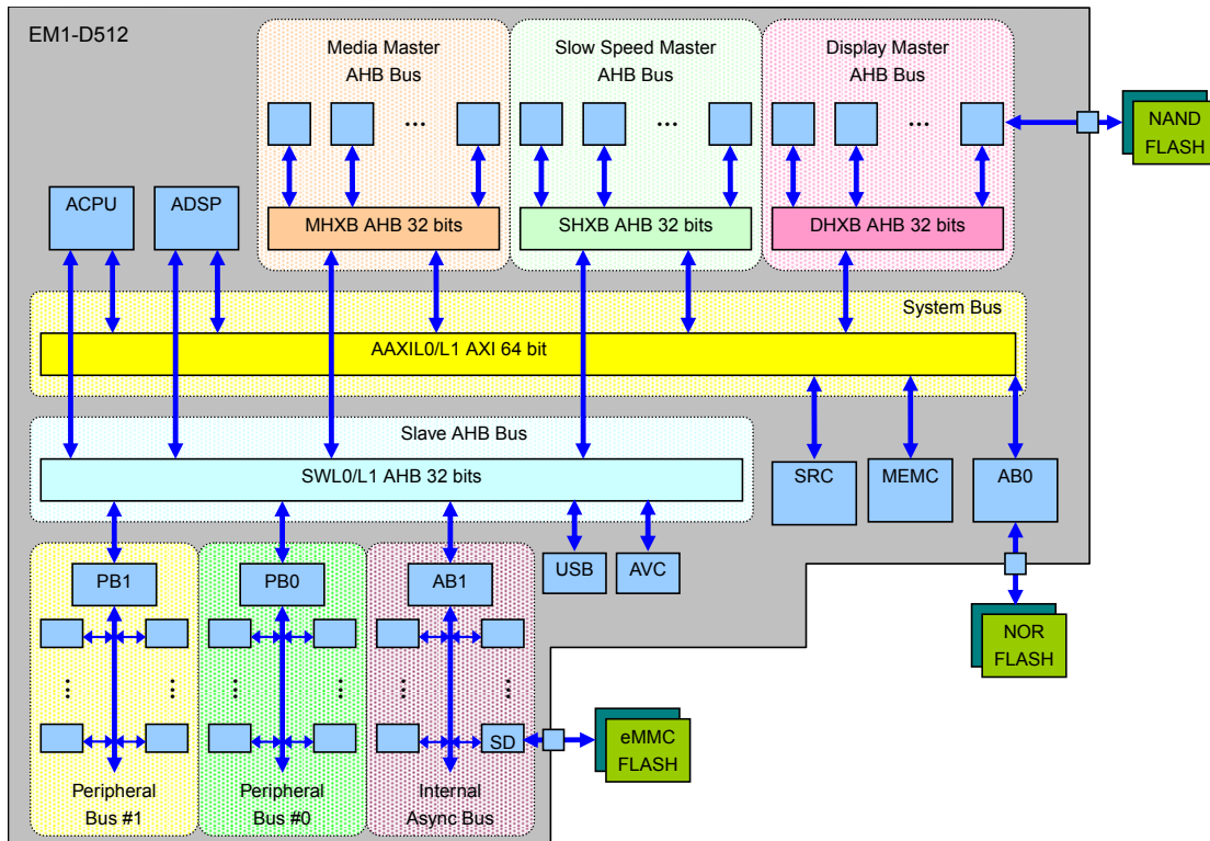
Figure 6-1. EM1-S Bus Configuration
