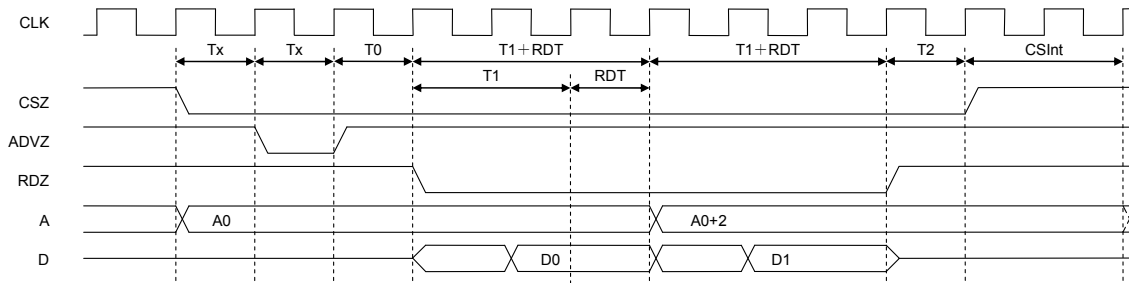
Figure E-8. Page Read Timing (Clock Ratio = 1:1)
