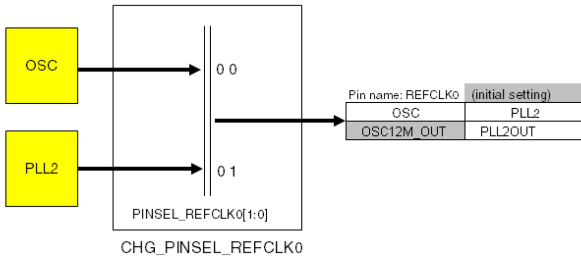
Figure 8-14. Selector Configuration of REFCLK0 Pin
