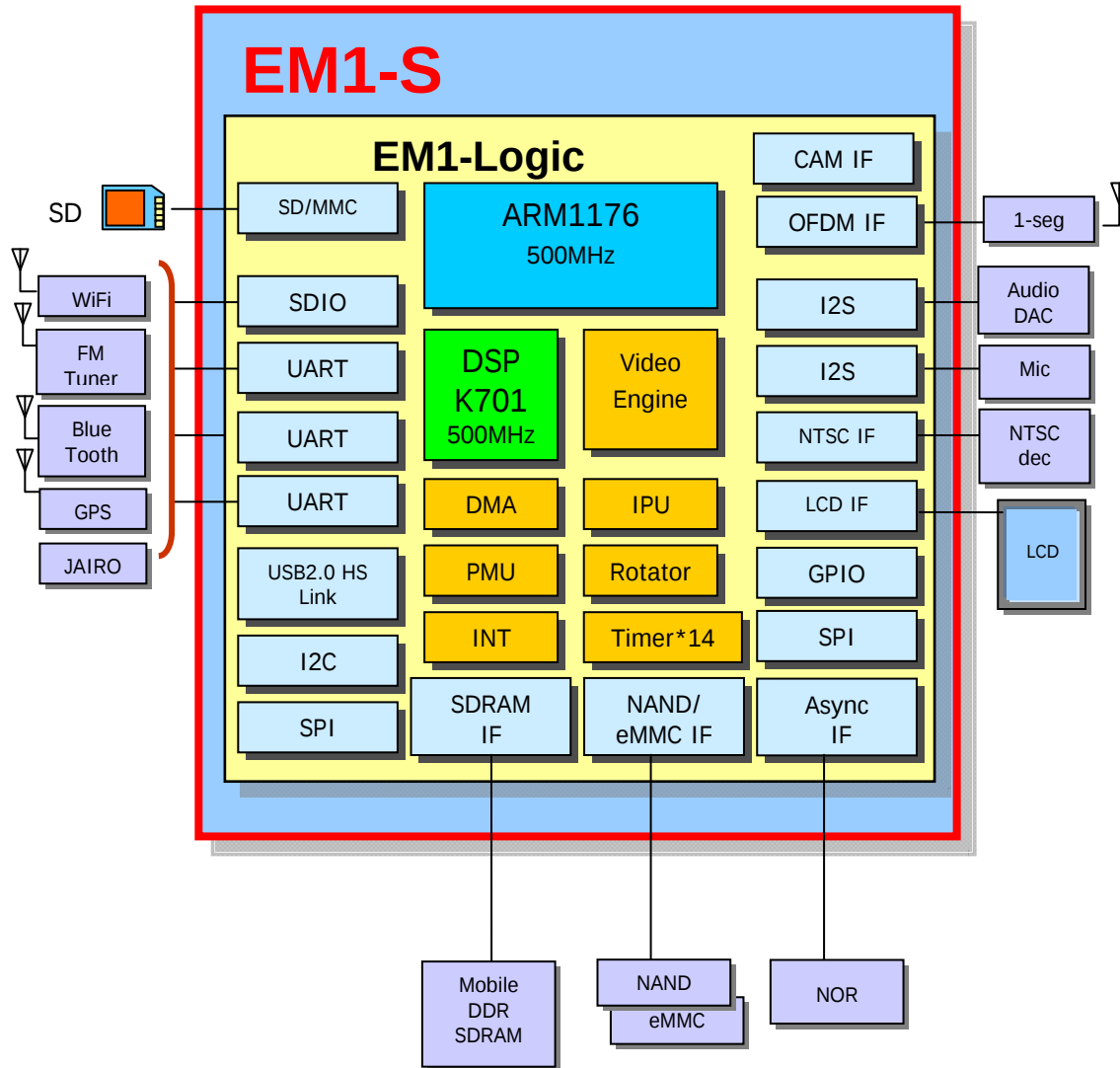
Figure 1-1. EM1-S System Configuration
