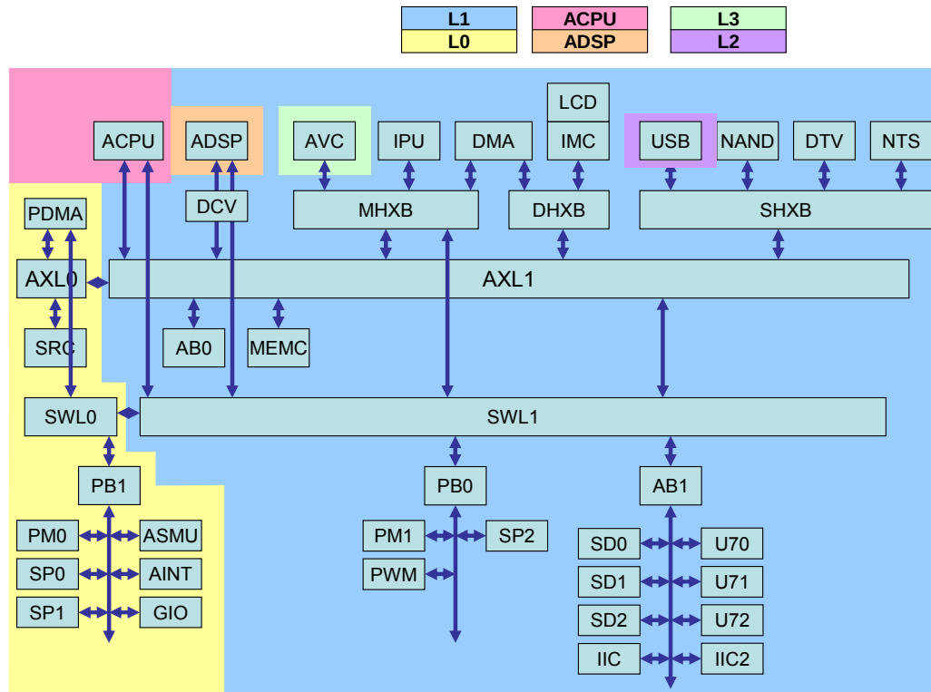
Figure 5-1. EM1-S Power Supply Separation Diagram
