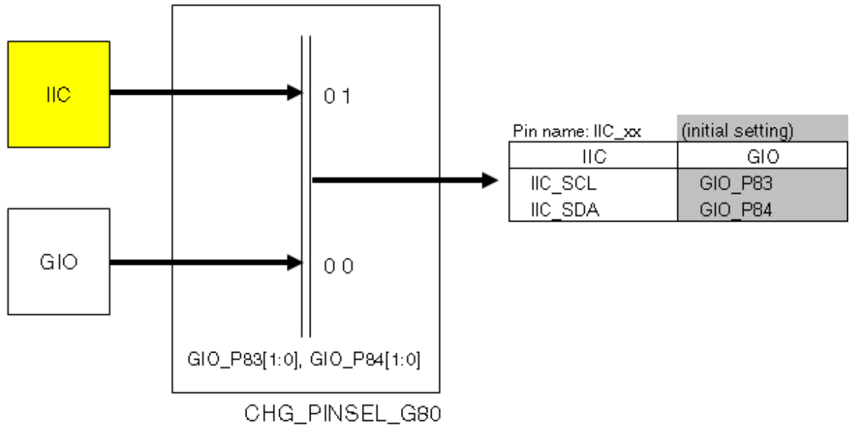
Figure 8-7. Selector Configuration of I 2 C Interface Alternate-Function Pins
