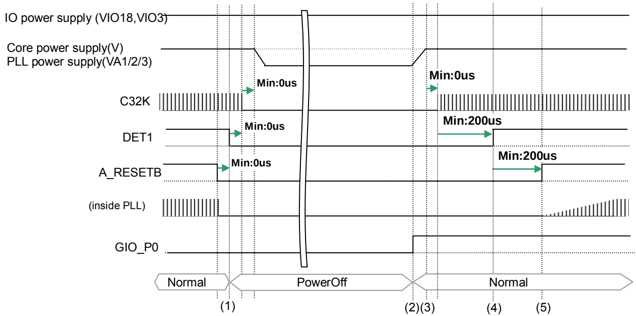
Figure 5-6. PowerOff Normal timing
