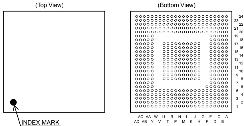
Figure 1-2. EM1-S Pin Layout
