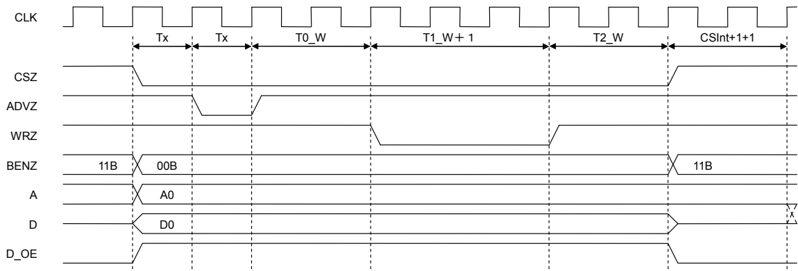
Figure E-4. Single Write Timing (Non Mux) (Clock Ratio = 1:1)
