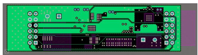
Figure 12. Layer 3 (Signal)
