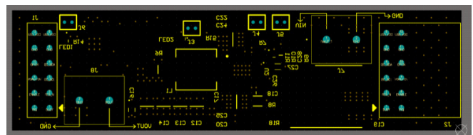
Figure 16. Bottom Overlay
