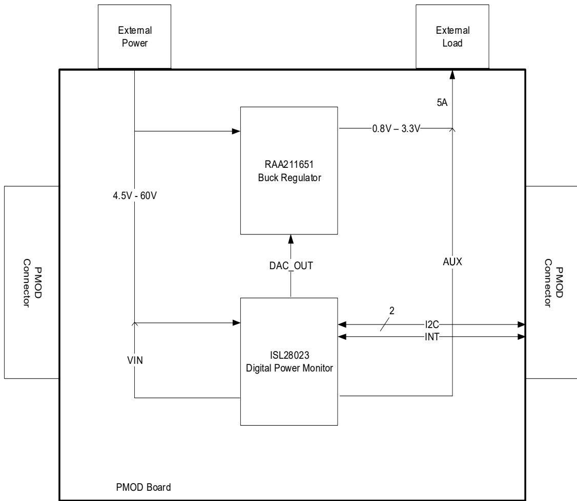
Figure 2. QCIOT-5APWRPOCZ Block Diagram
