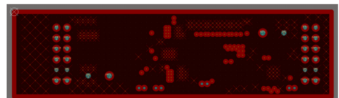
Figure 14. Layer 5 (GND)
