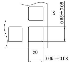
Detail F
