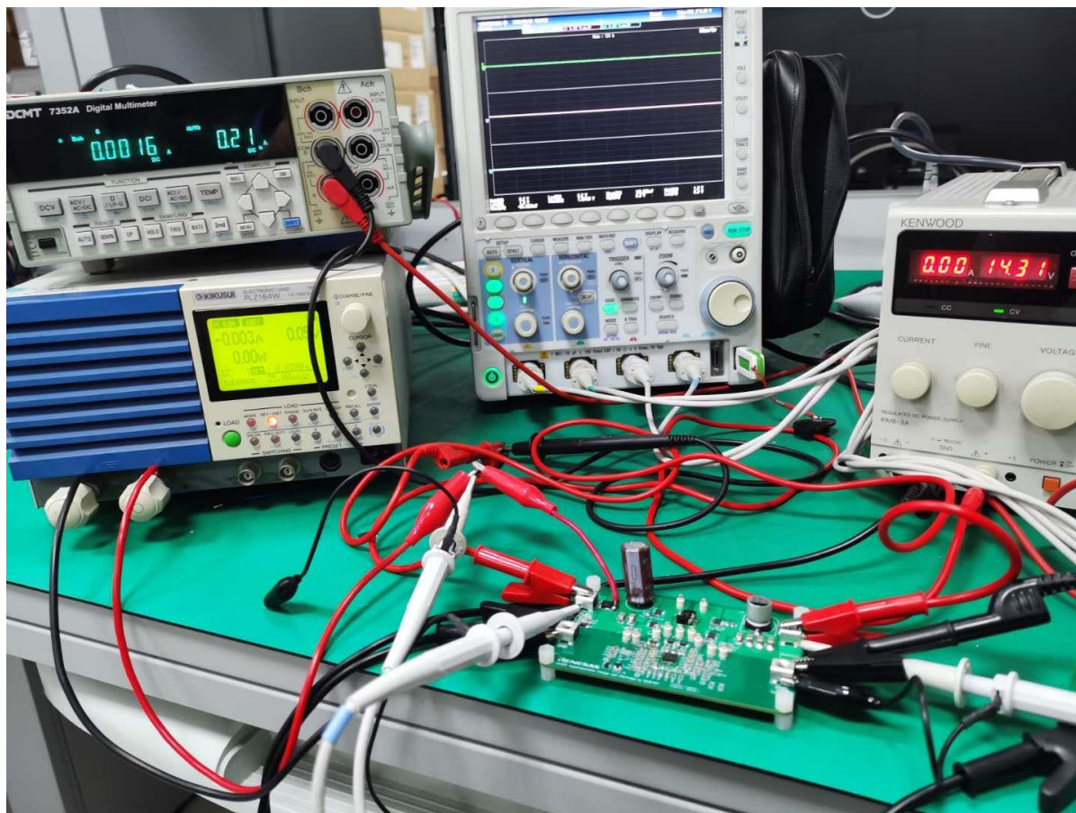
Figure 5 Test Environment
