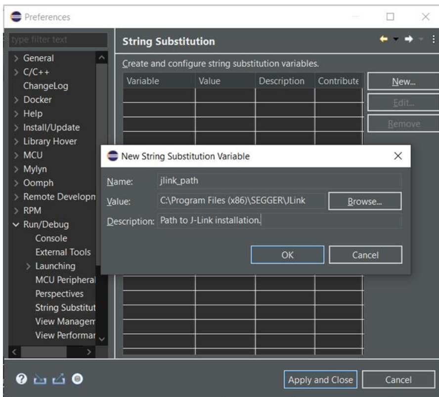
Figure 33: Install path of J-Link in Eclipse
