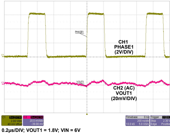
FIGURE 5. PWM1 SWITCHING AND RIPPLE WAVEFORMS AT NO LOAD
