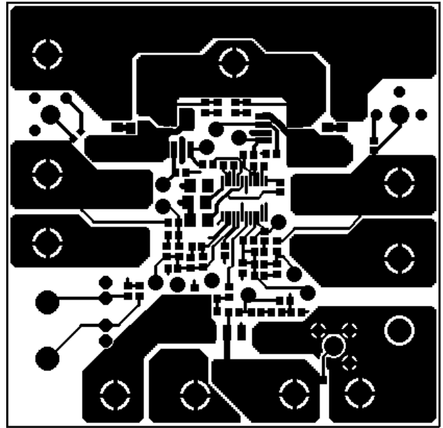
FIGURE 9. TOP LAYER
