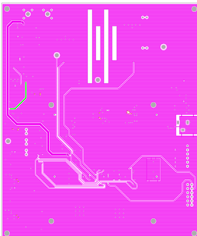
Figure 40. Layer 3
