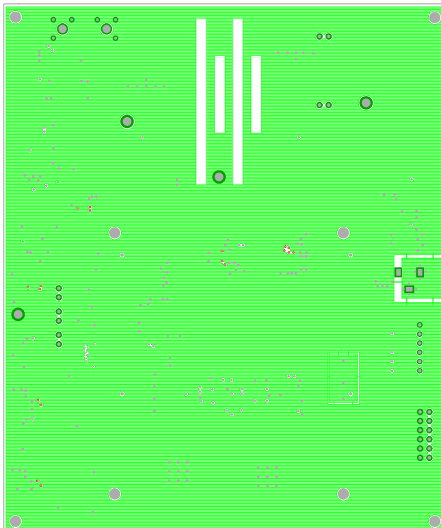
Figure 39. Layer 2
