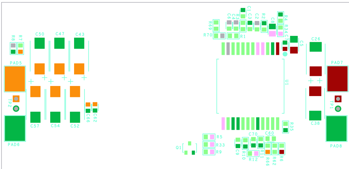
Figure 17. Silkscreen Bottom Layer
