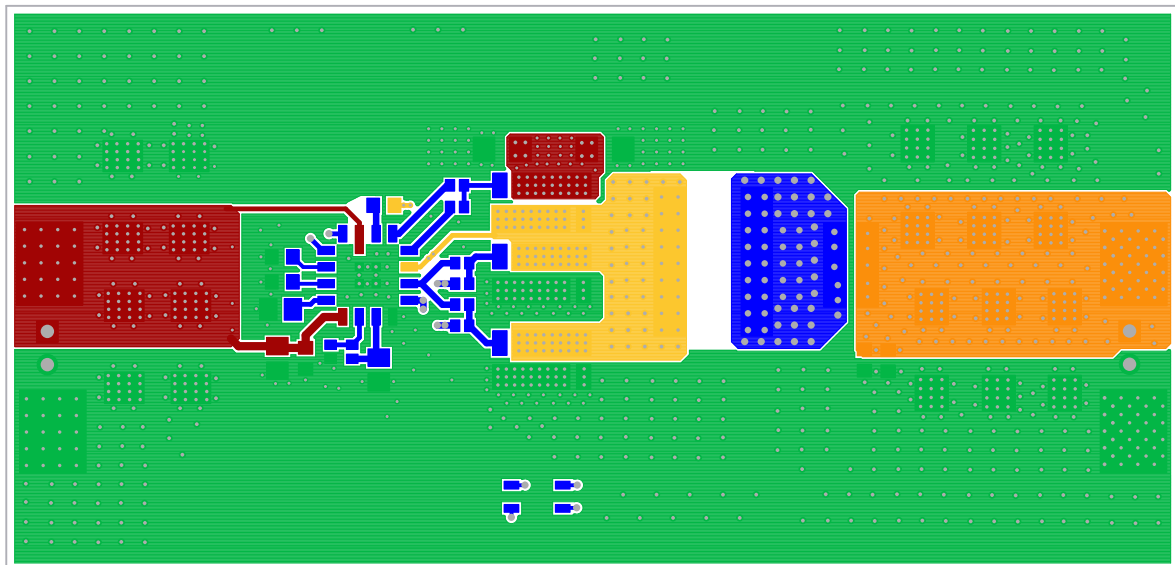
Figure 9. Top Layer
