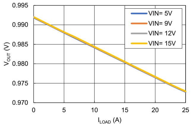
Figure 19. Droop Regulation for Various V_{IN}
