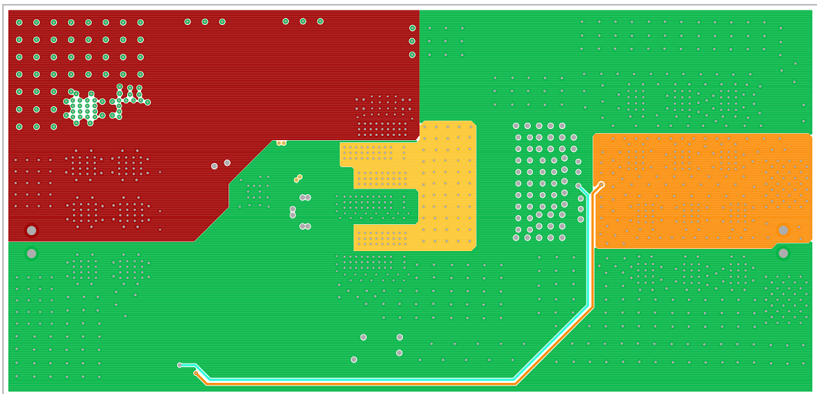
Figure 11. Layer 3
