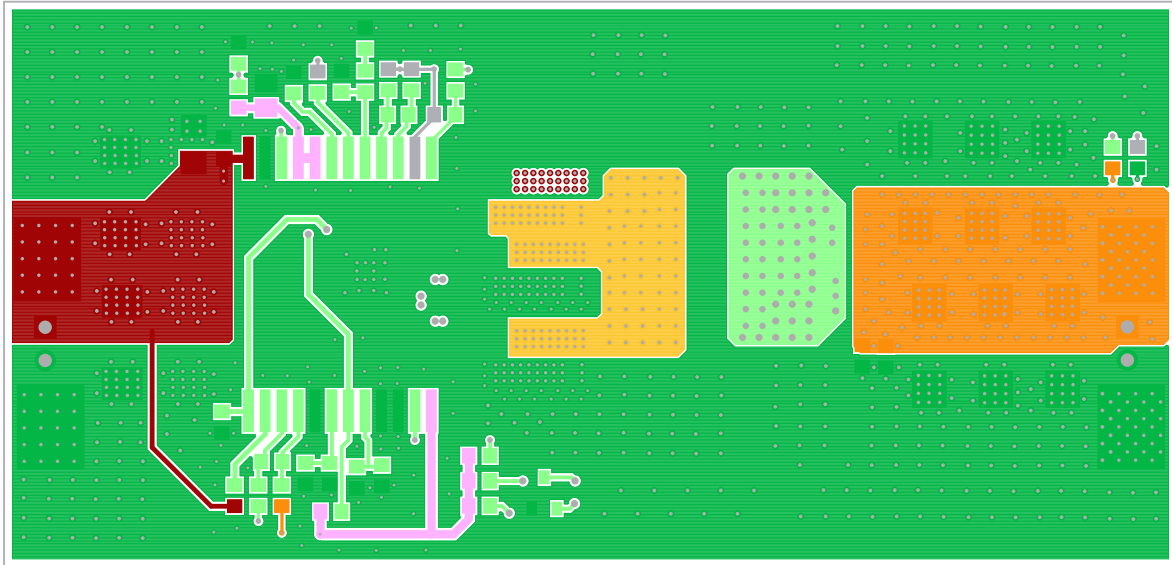
Figure 16. Bottom Layer
