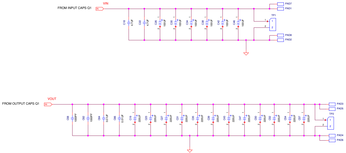
Figure 7. ISL73847SEHDEMO5Z Schematic Page 2
