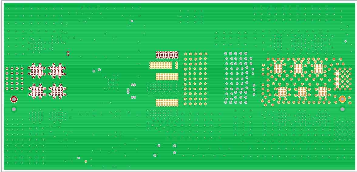
Figure 14. Layer 6
