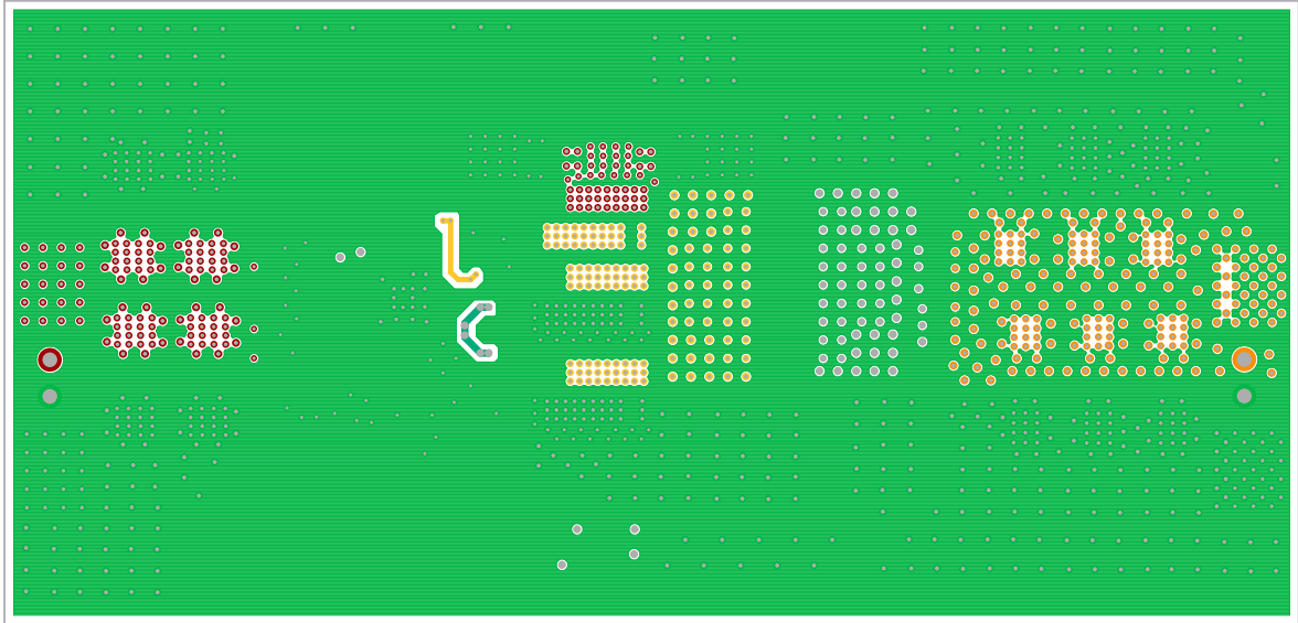
Figure 10. Layer 2
