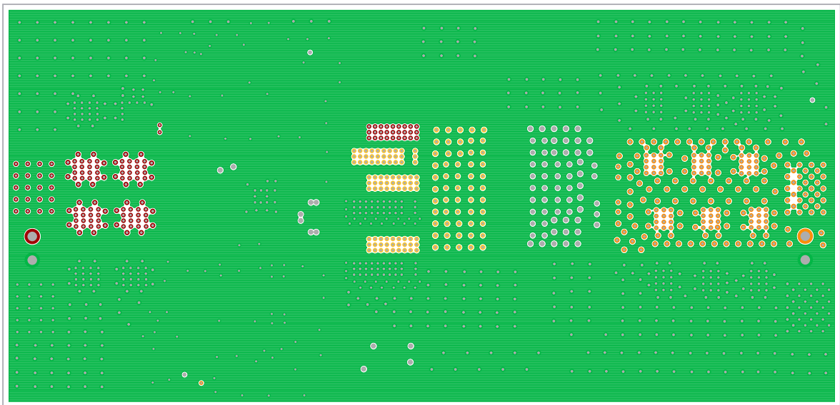
Figure 13. Layer 5
