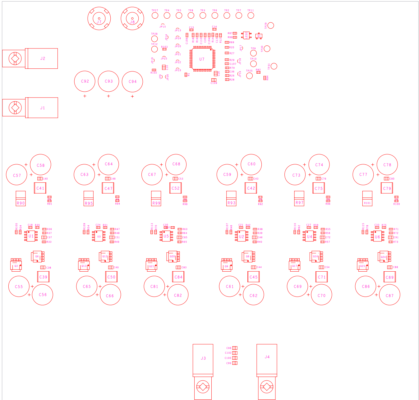
FIGURE 12. ASSEMBLY TOP
