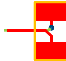
FIGURE 9. RECOMMENDED LAYOUT PATTERN FOR CURRENT SENSE TRACES REGULATOR
