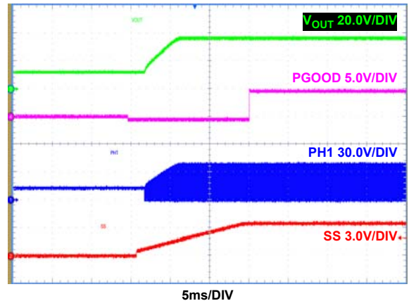
FIGURE 25. SOFT-START, DE+PHDRP MODE (DE/PHDRP = FLOAT), I_{OUT} = 8A
