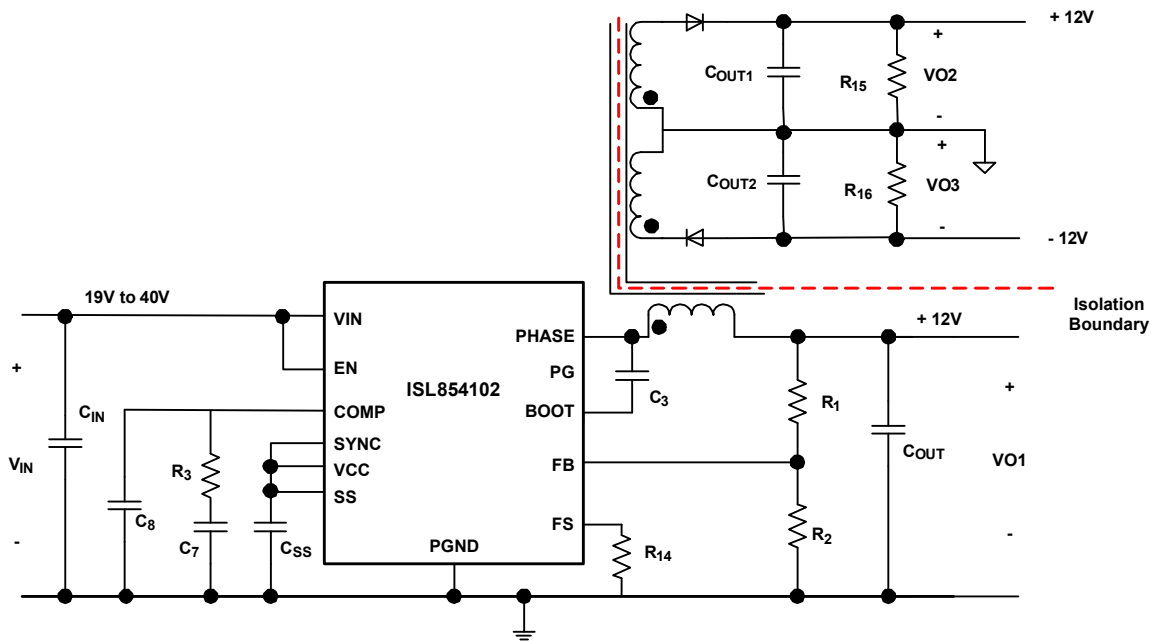
Figure 1. Block Diagram
