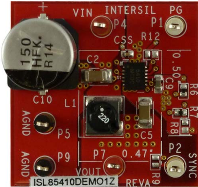
FIGURE 2. ISL85410DEMO1Z DEMONSTRATION BOARD (TOP)
