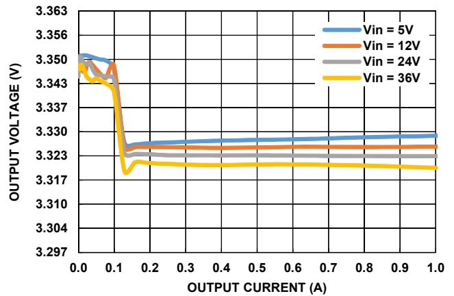
FIGURE 20. V_{OUT} REGULATION vs LOAD, PFM, V_{OUT} = 3.3V
