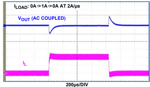
FIGURE 22. LOAD TRANSIENT, PWM
