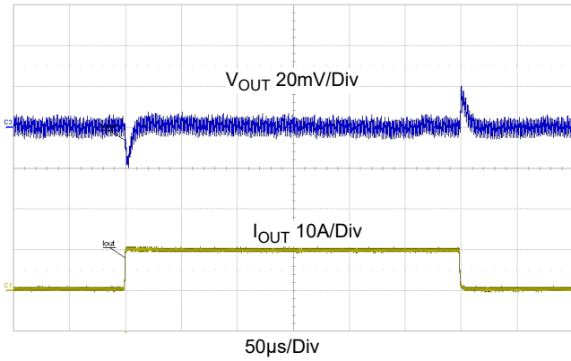
Figure 29. Transient Response, V_{IN} = 12V , V_{OUT} = 1.8V , 0A to 10A to 0A, 5A/µs Step Load, C_{OUT} = 7 \times 47\mu F Ceramic + 2x470µF Polymer Capacitor
