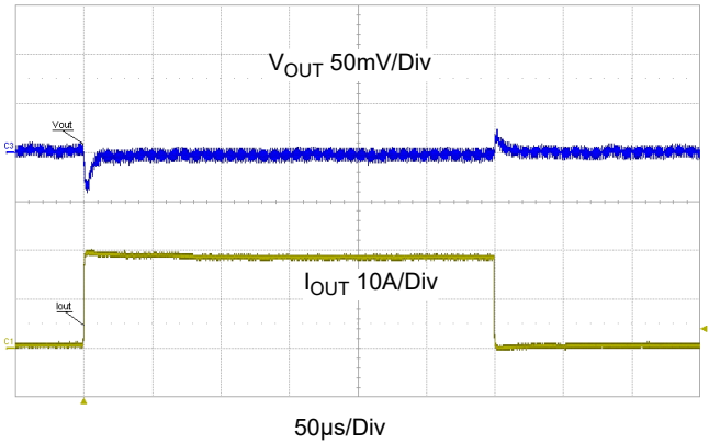
Figure 30. Transient Response, V_{IN} = 12V , V_{OUT} = 3.3V , 0A to 20A to 0A, 5A/µs Step Load, C_{OUT} = 15 \times 47\mu F Ceramic + 2x470µF Polymer Capacitor
