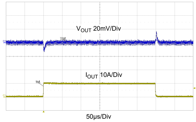
Figure 26. Transient Response, V_{IN} = 12V , V_{OUT} = 0.8V , 0A to 15A to 0A, 5A/\mu s Step Load, C_{OUT} = 10 \times 47\mu F Ceramic + 2 \times 470\mu F Polymer Capacitor
