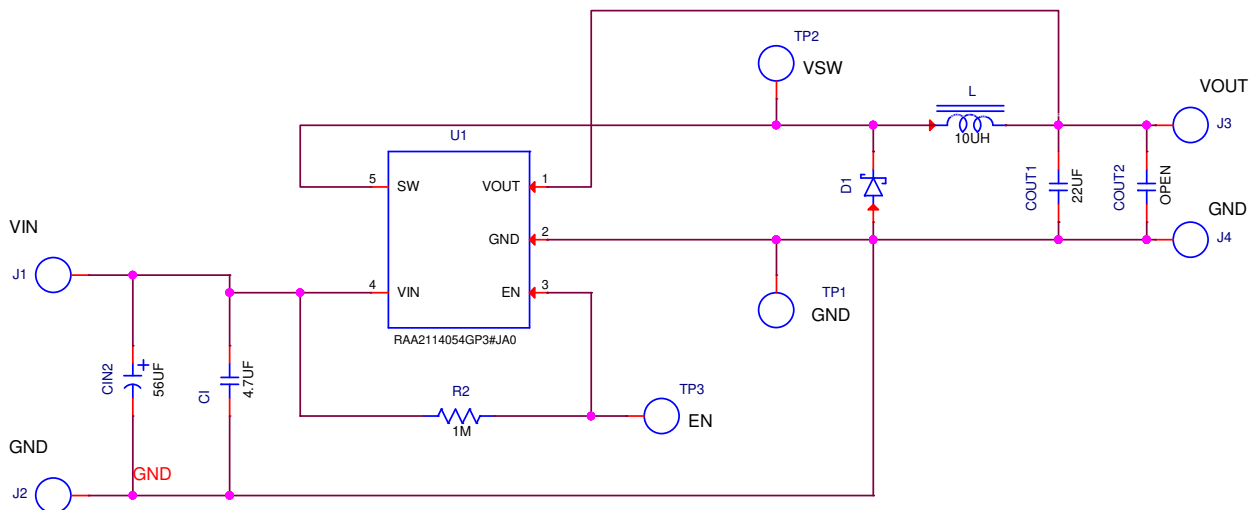
Figure 5. RTKA211405DE0000BU Schematic
