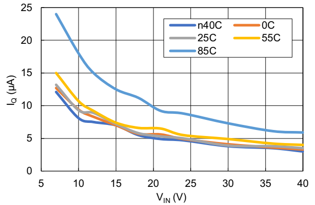
Figure 19. I_Q vs V_{IN} (In Regulation: No Load)
