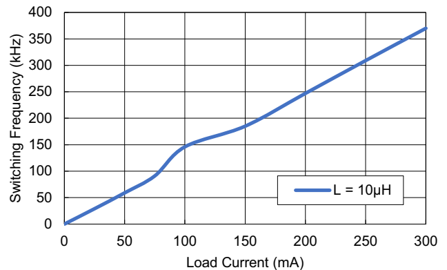
Figure 3. Switching Frequency (VIN 24V) vs Load Current
