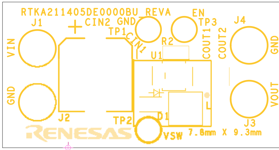
Figure 6. Silkscreen Top
