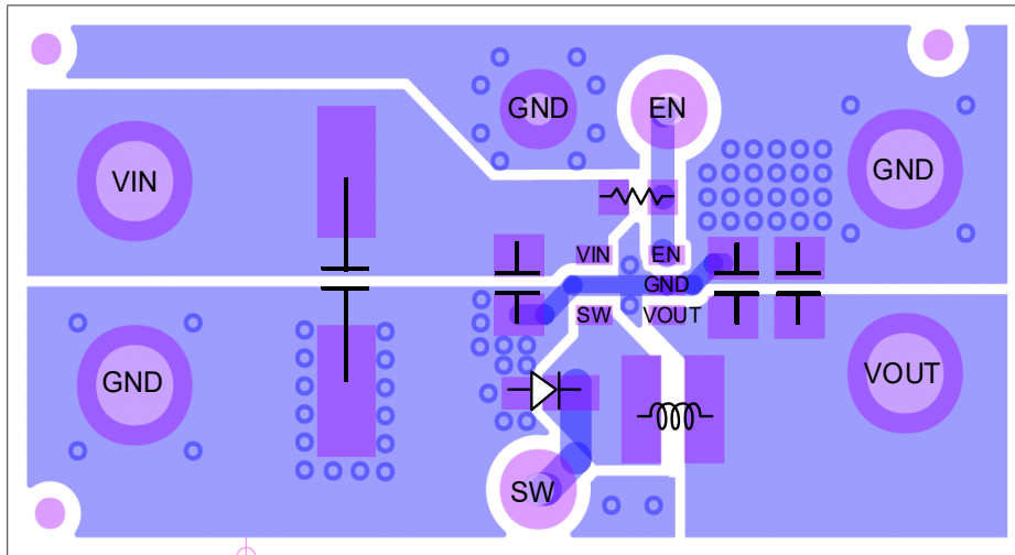
Figure 7. Top Layer
