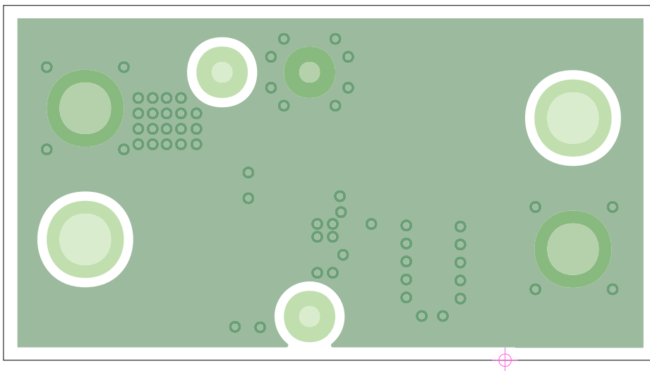
Figure 8. Bottom Layer
