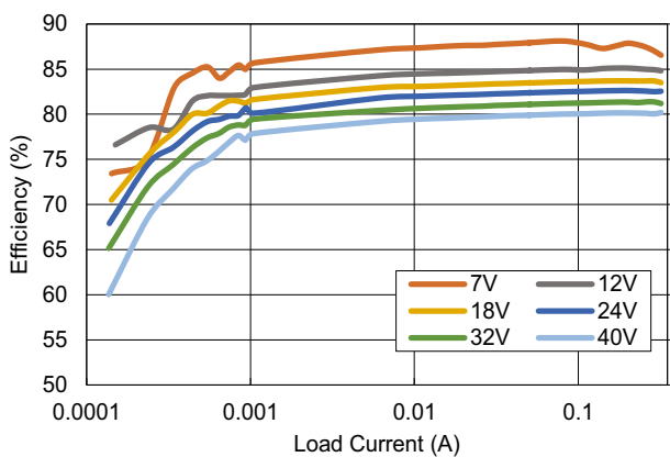
Figure 20. Efficiency
