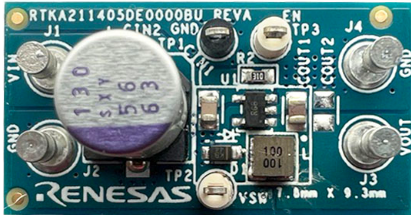
Figure 4. RTKA211405DE0000BU Evaluation Board (Top)
