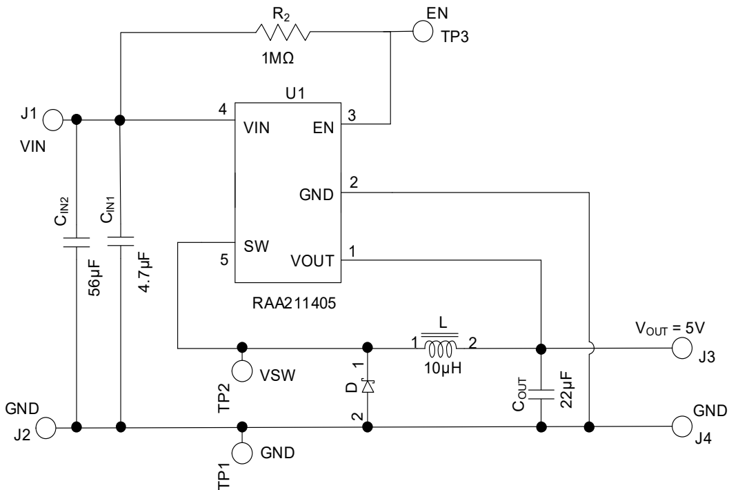
Figure 1. RTKA211405DE0000BU Block Diagram
