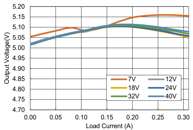
Figure 21. Load Regulation
