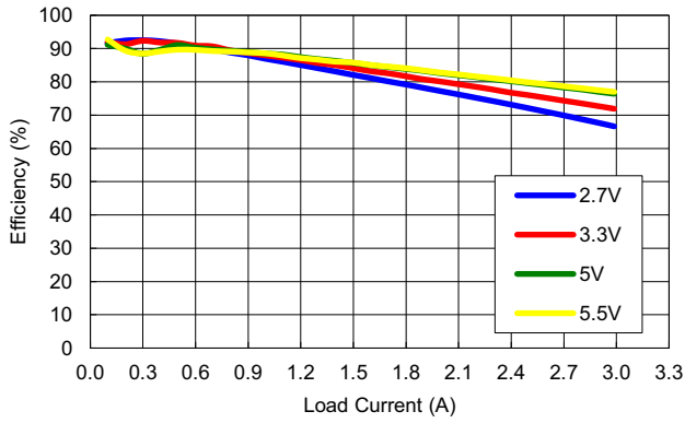
Figure 14. Efficiency vs Load, V_{OUT} = 1.2V , 85^{\circ}C
