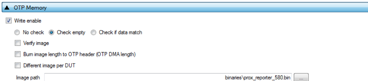
Figure 71: OTP Memory - DA1458x
