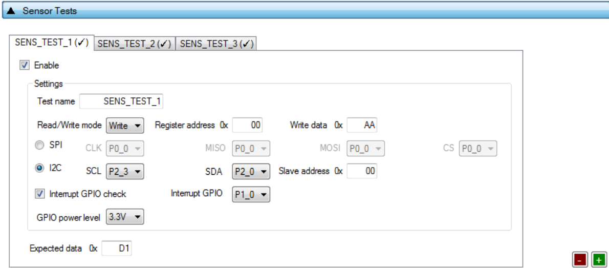
Figure 95: Sensor Test - DA1468x
