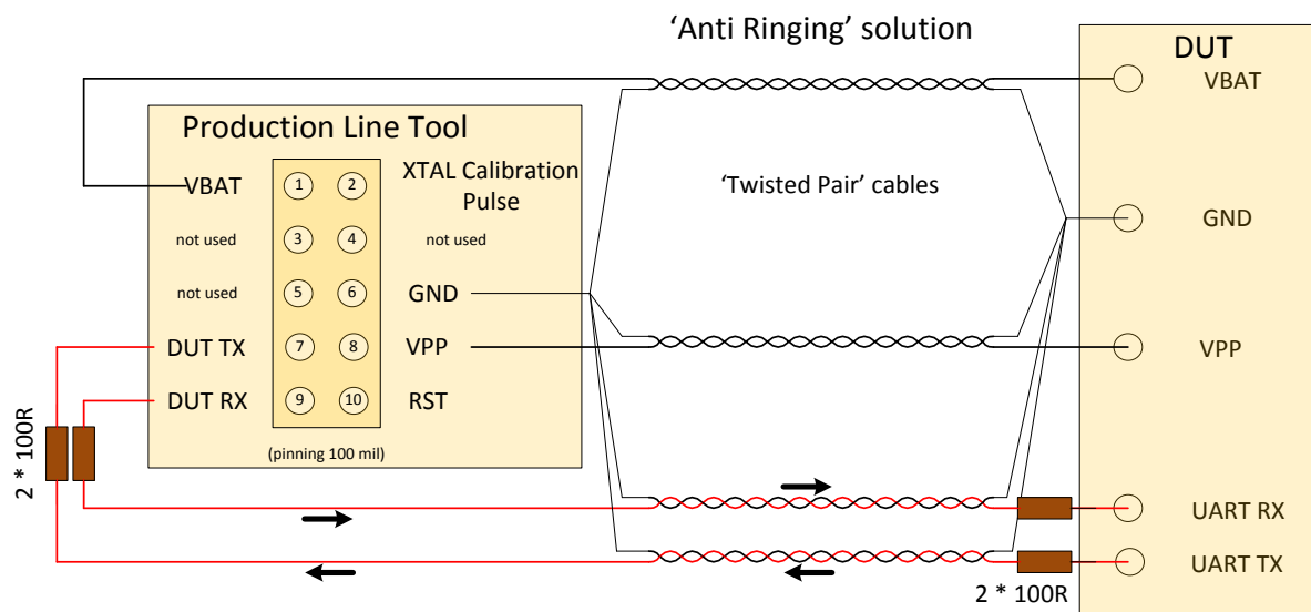
Figure 171: Anti-Ringing Solution
