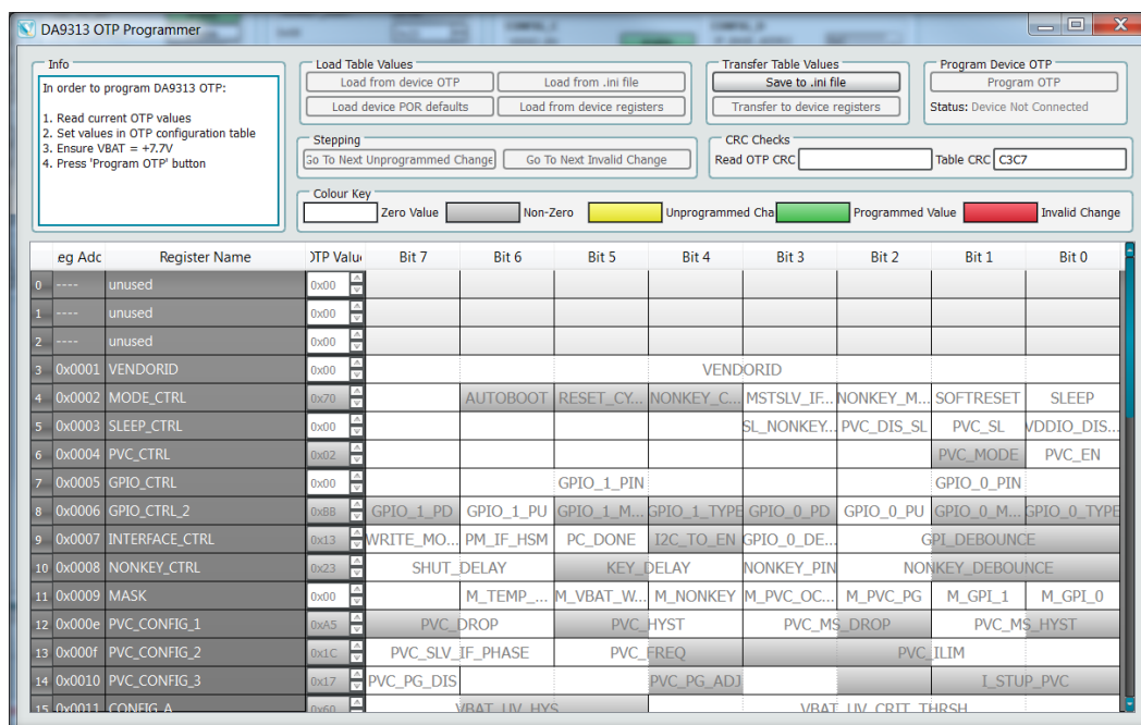
Figure 25: OTP Programmer
