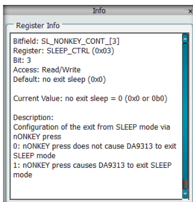
Figure 23: Info
