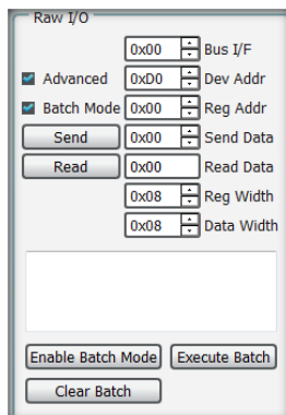
Figure 16: Raw I/O
