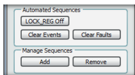
Figure 17: Automated Sequence
