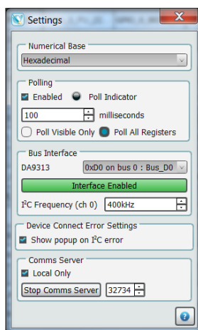
Figure 24: Settings
