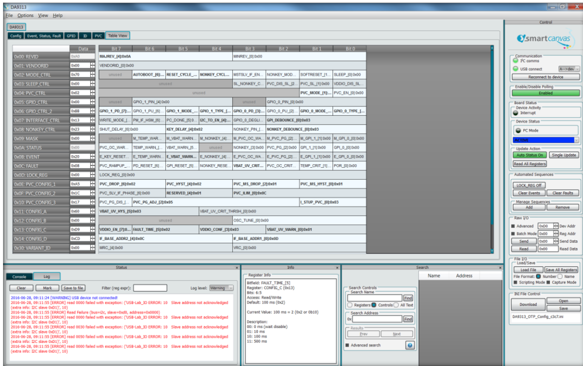
Figure 12: Table View
