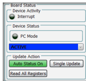
Figure 15: Board Status
