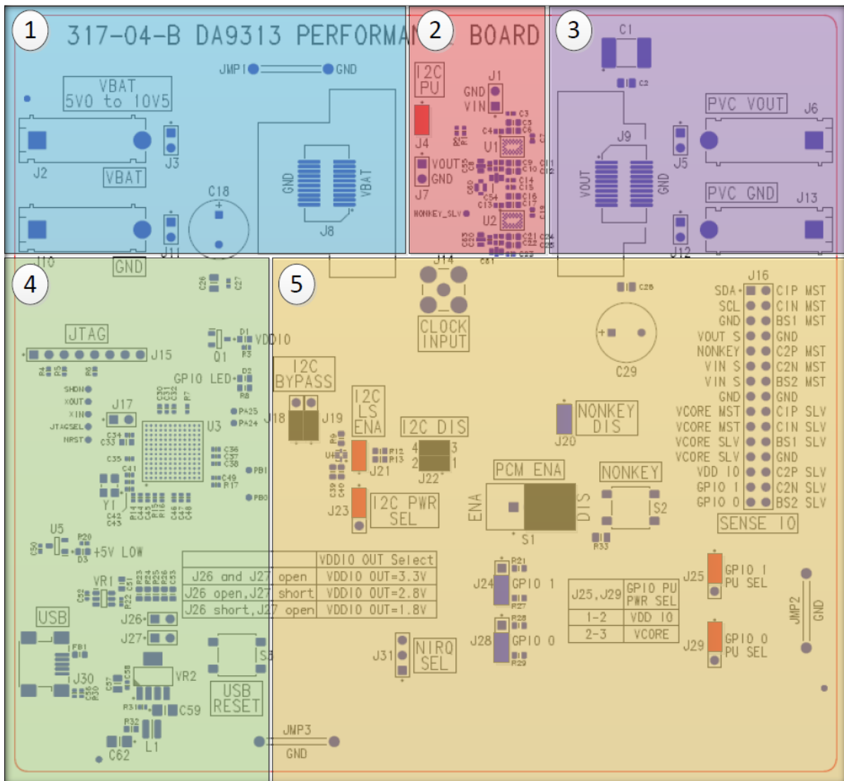
Figure 2: DA9313 Performance Board Sections (317-04-B Shown)
