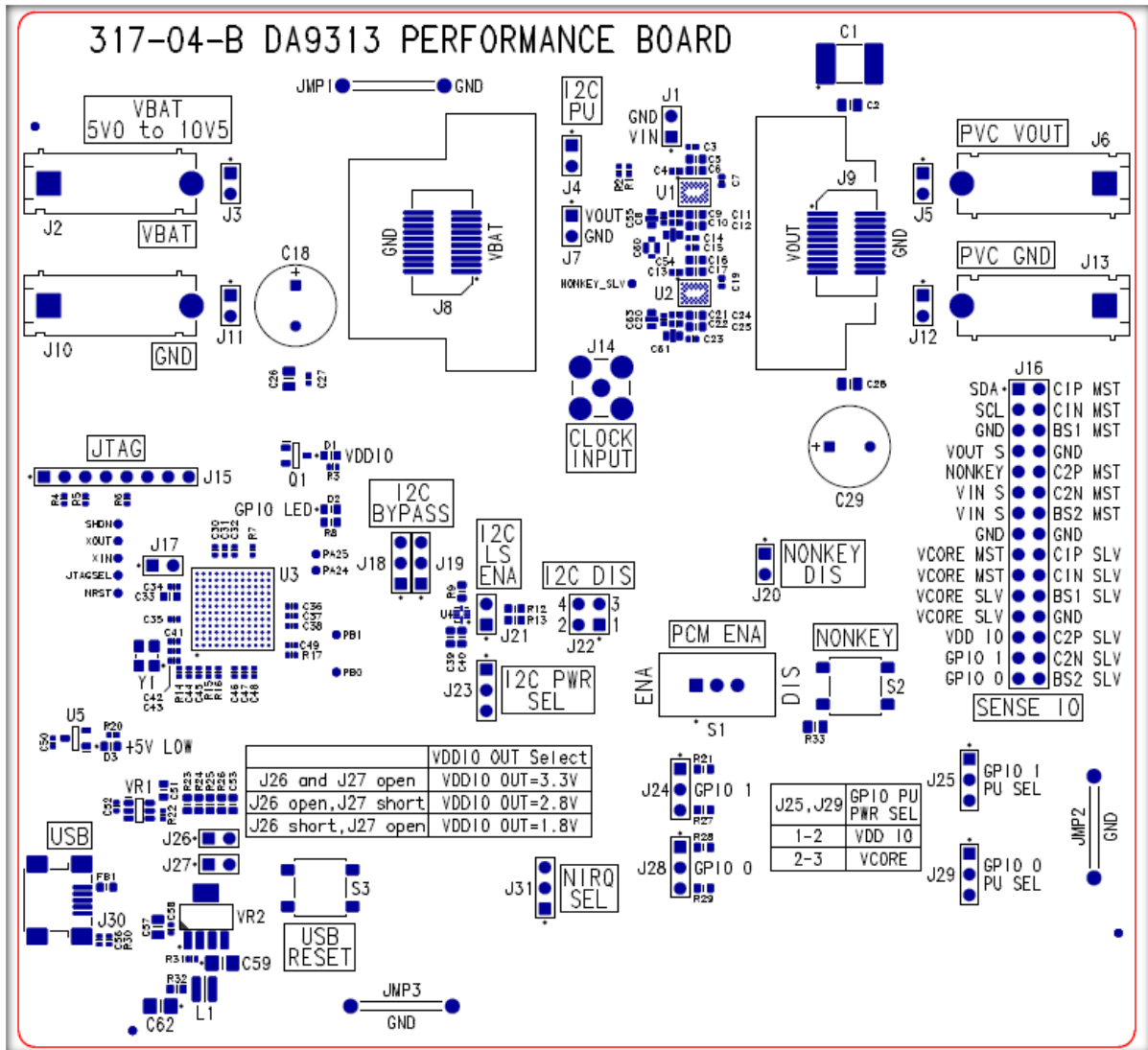
Figure 3: DA9313 Performance Board Default Link Positions (317-04-B Shown)
