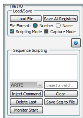
Figure 20: File I/O
