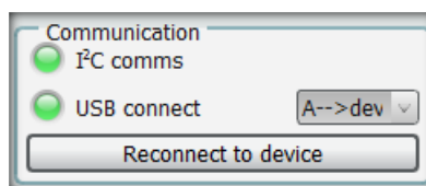
Figure 13: Communication Control
