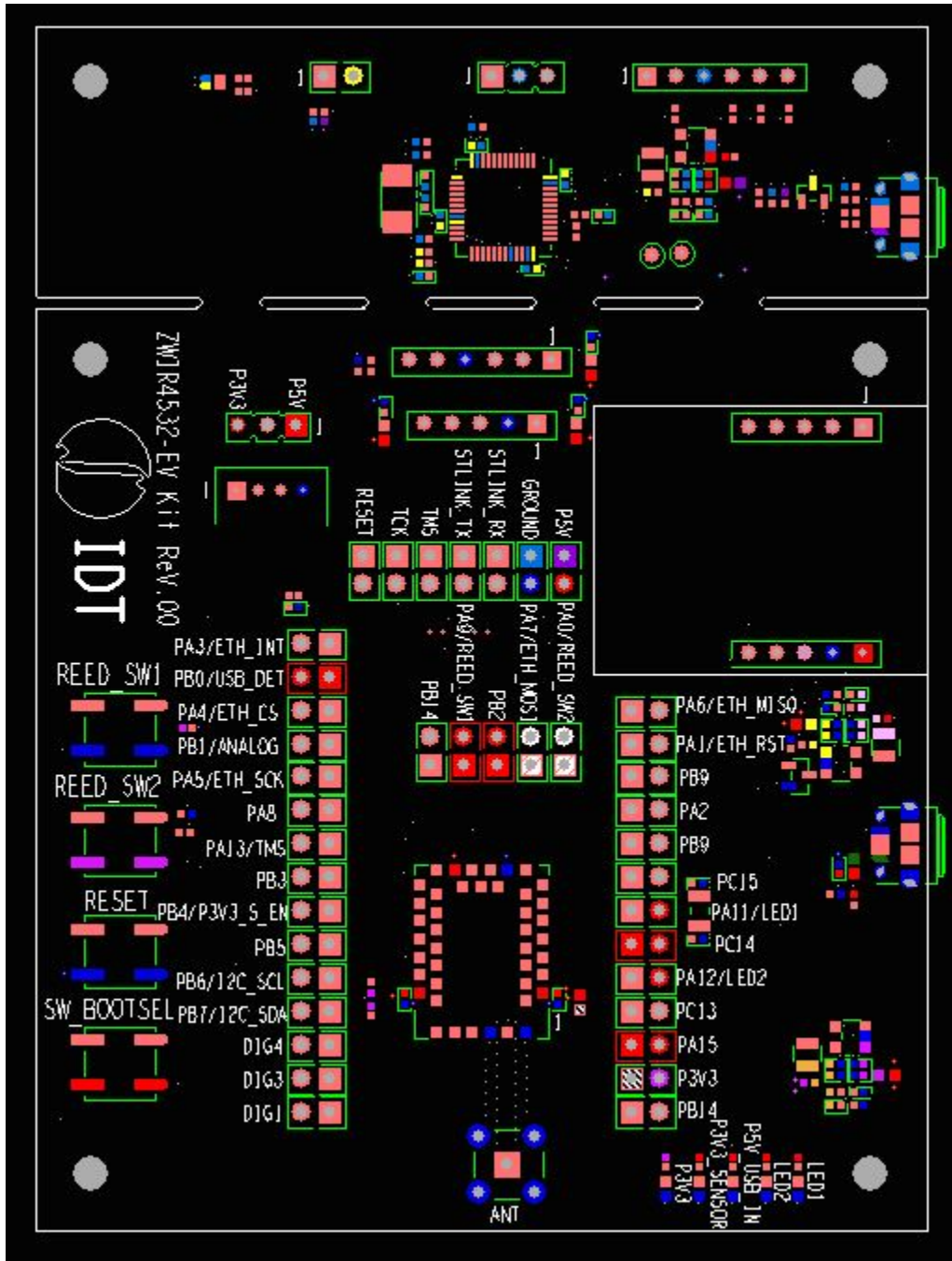
Figure 2. Jumper Locations
