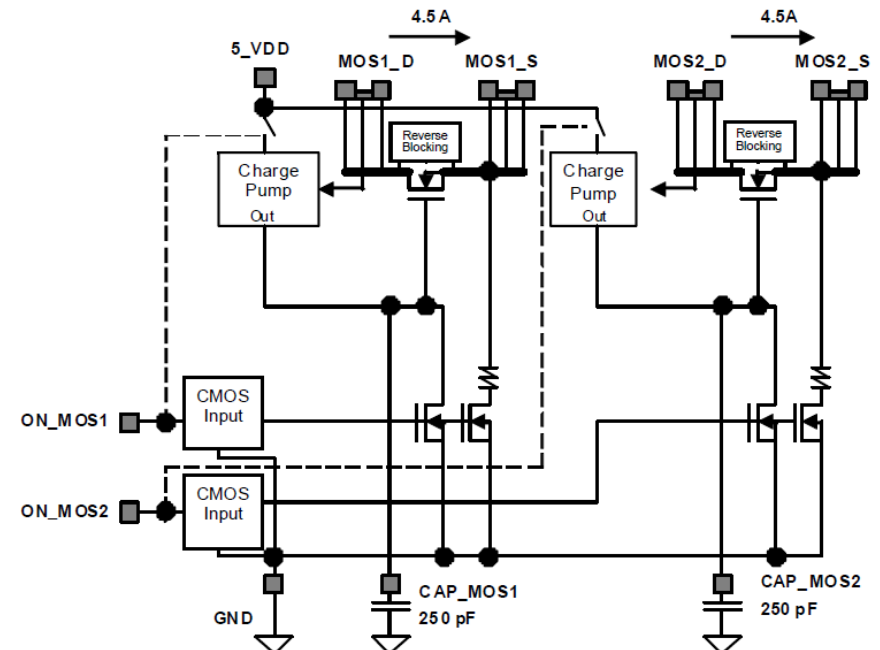
Figure 1: SLG59M1606V Block Diagram
