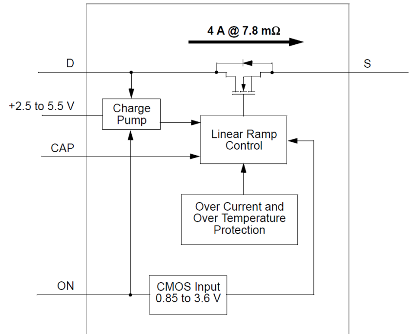
Figure 1: SLG59M309V Block Diagram
