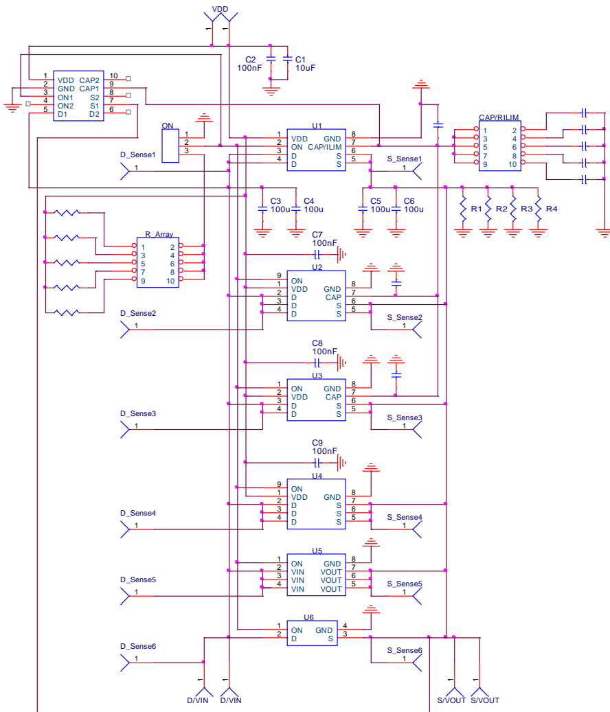
Figure 4. SLG59M309V Connection Circuit
