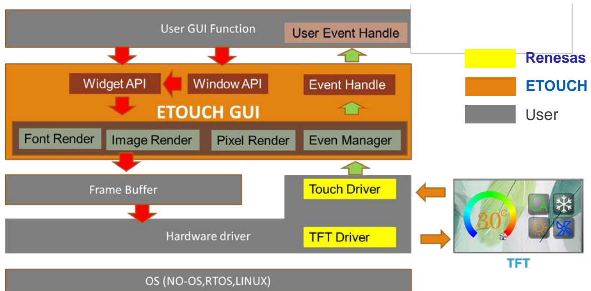
Figure: Etouch GUI Framework
