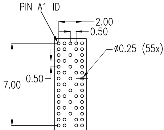
RECOMMENDED LAND PATTERN DIMENSION (NSMD) (TOP VIEW)
