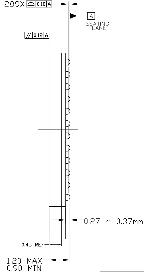
SIDE VIEW
