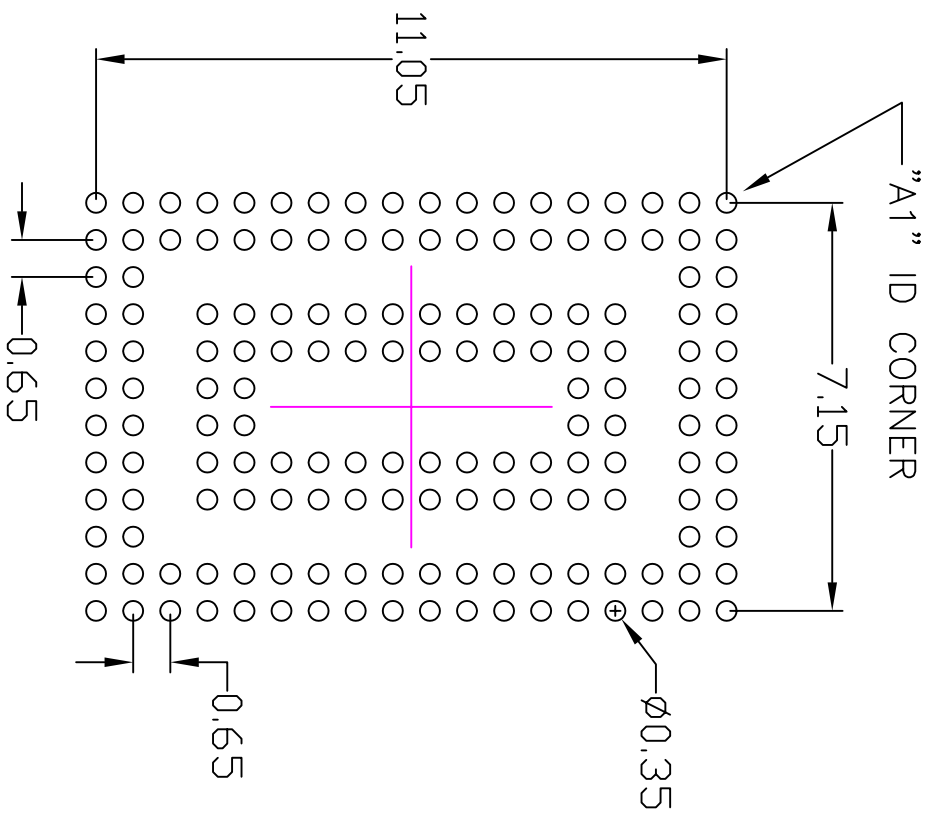
RECOMMENDED LAND PATTERN DIMENSION
