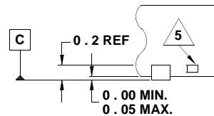
DETAIL "X"
