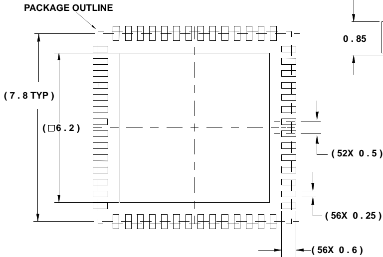
TYPICAL RECOMMENDED LAND PATTERN
