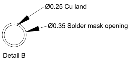
Detail B
