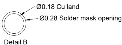
RECOMMENDED LAND PATTERN (PCB Top View, NSMD Design)
