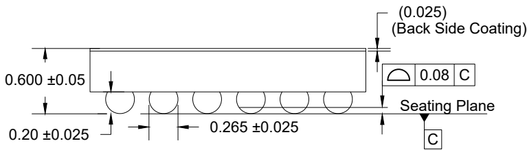
SIDE VIEW
