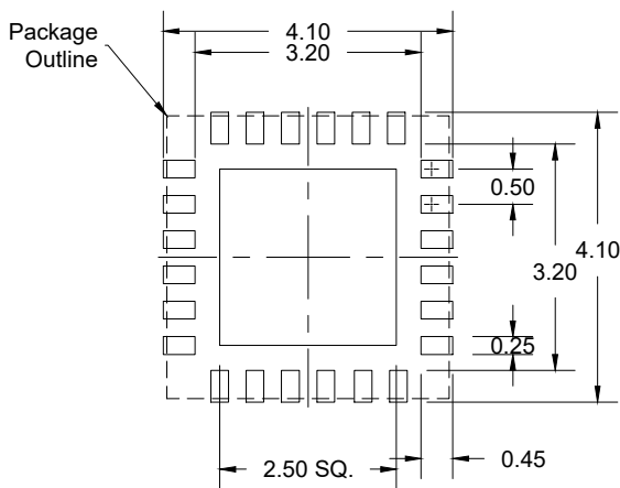
RECOMMENDED LAND PATTERN (PCB Top View)
