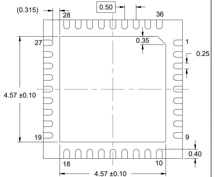
BOTTOM VIEW
