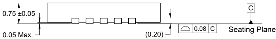
SIDE VIEW
