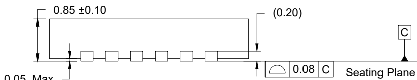
SIDE VIEW
