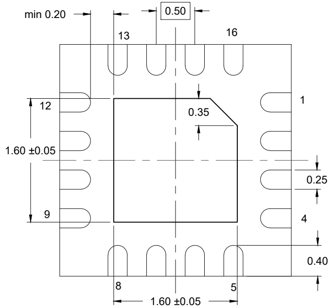
BOTTOM VIEW
