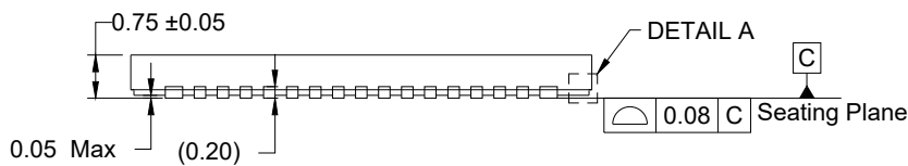
SIDE VIEW
