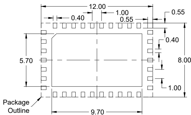
RECOMMENDED LAND PATTERN (PCB Top View)
