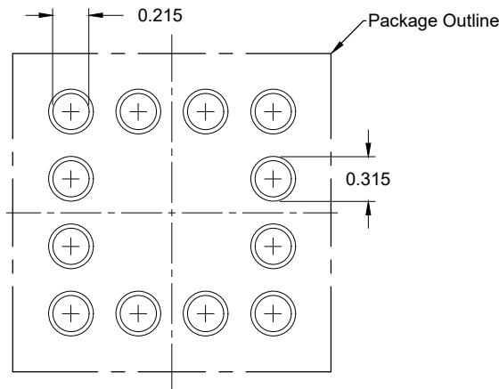
Ⓐ NSMD Recommended Land Pattern
