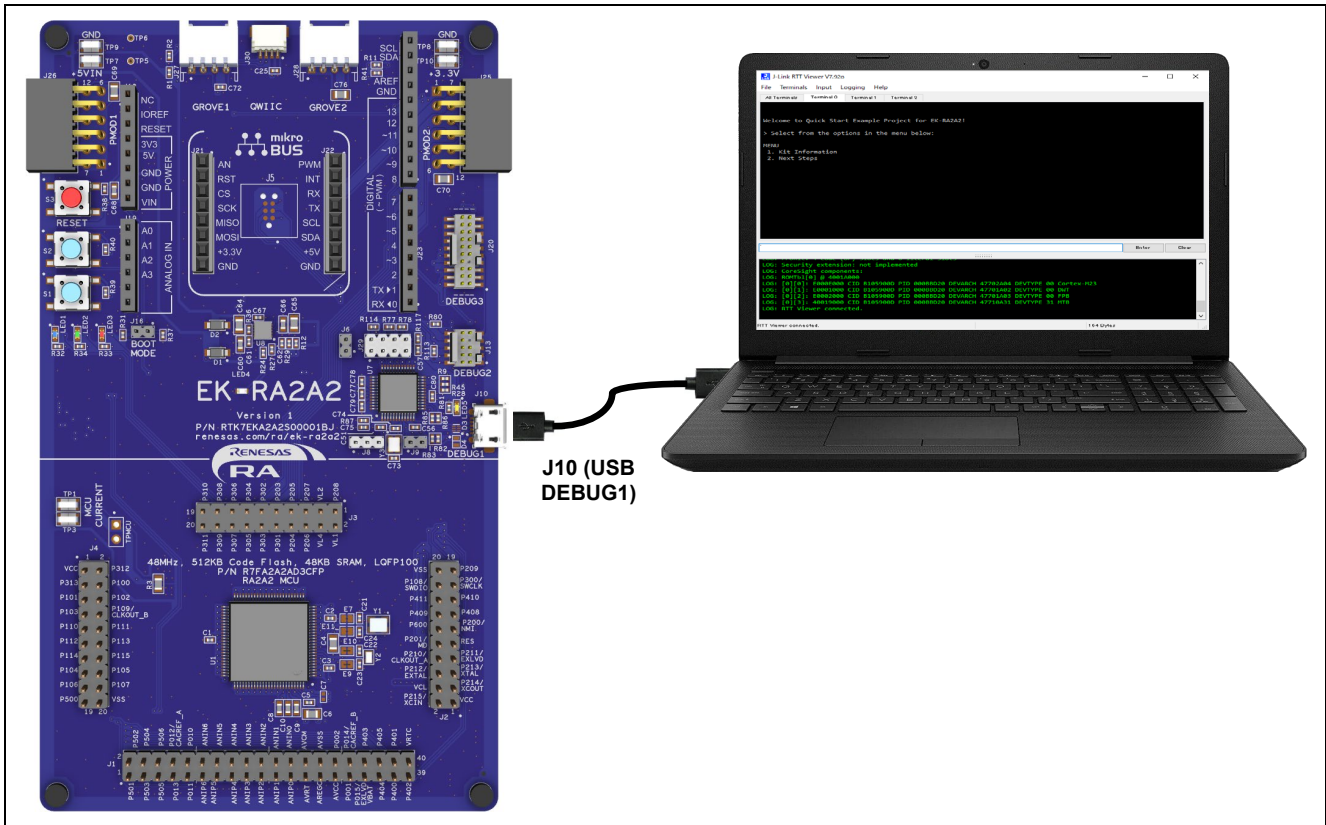
Figure 3. Connecting the EK-RA2A2 Board to the Host PC via USB Debug Port J10
