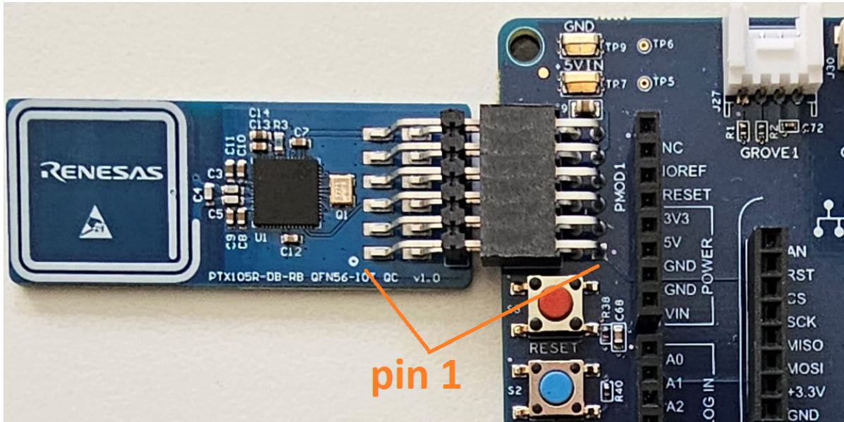
Figure 3. Connecting the PTX105RQC and EK-RA2E1 Boards
