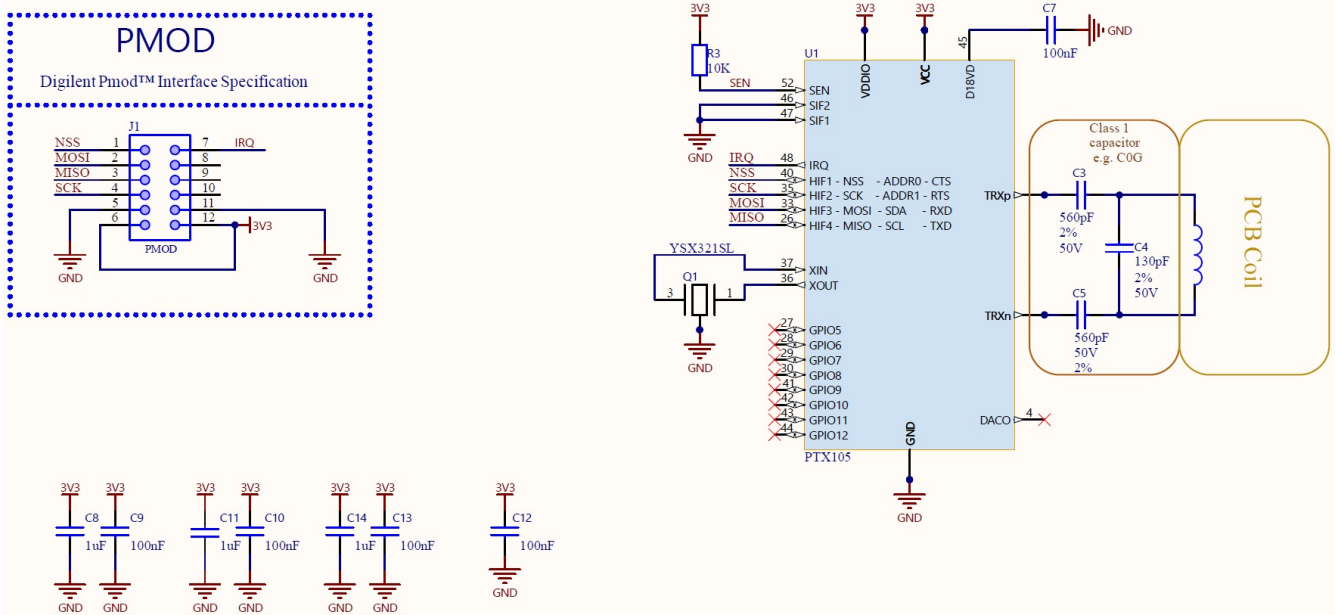
Figure 11. PTX105R-DB-RB QFN56-IOT QC Schematic
